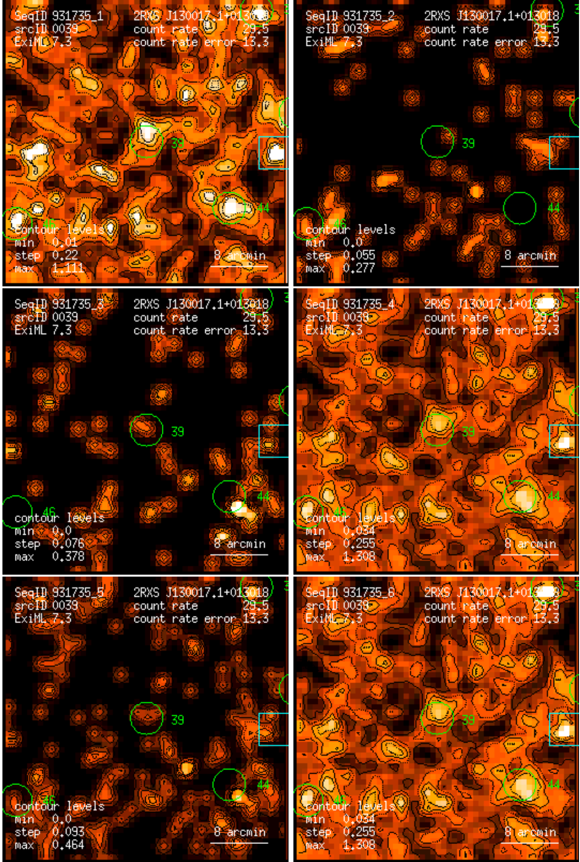
Figure 39: RASS 931735: detection 0039: band rate images, Gaussian filter: (1) PSPC channels 11 – 41, (2) 52 – 90, (3) 91 – 201, (4) 11 – 235, (5) 52 – 201, (6) 11 – 201. Broad band rates in counts/ks. Band rate contour levels in counts/ks/arcmin 2 .
