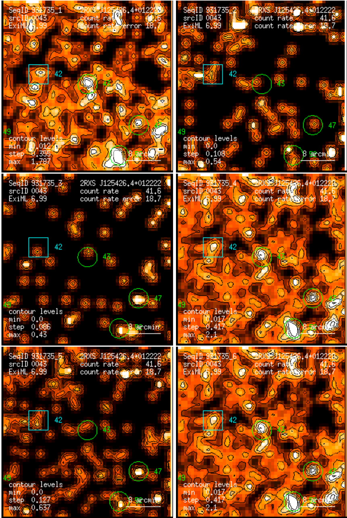
Figure 43: RASS 931735: detection 0043: band rate images, Gaussian filter: (1) PSPC channels 11 – 41, (2) 52 – 90, (3) 91 – 201, (4) 11 – 235, (5) 52 – 201, (6) 11 – 201. Broad band rates in counts/ks. Band rate contour levels in counts/ks/arcmin 2 .
