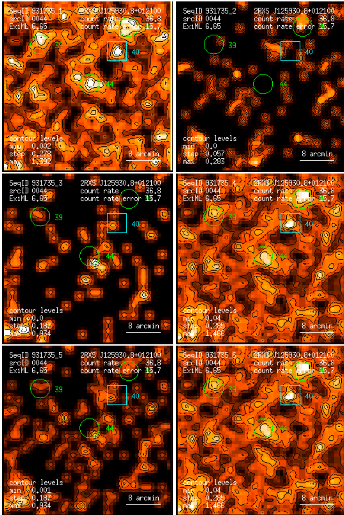
Figure 44: RASS 931735: detection 0044: band rate images, Gaussian filter: (1) PSPC channels 11 – 41, (2) 52 – 90, (3) 91 – 201, (4) 11 – 235, (5) 52 – 201, (6) 11 – 201. Broad band rates in counts/ks. Band rate contour levels in counts/ks/arcmin 2 .
