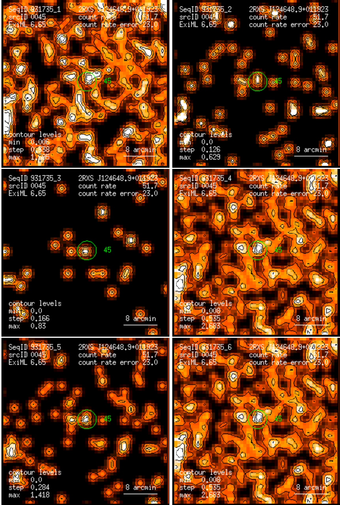
Figure 45: RASS 931735: detection 0045: band rate images, Gaussian filter: (1) PSPC channels 11 – 41, (2) 52 – 90, (3) 91 – 201, (4) 11 – 235, (5) 52 – 201, (6) 11 – 201. Broad band rates in counts/ks. Band rate contour levels in counts/ks/arcmin 2 .
