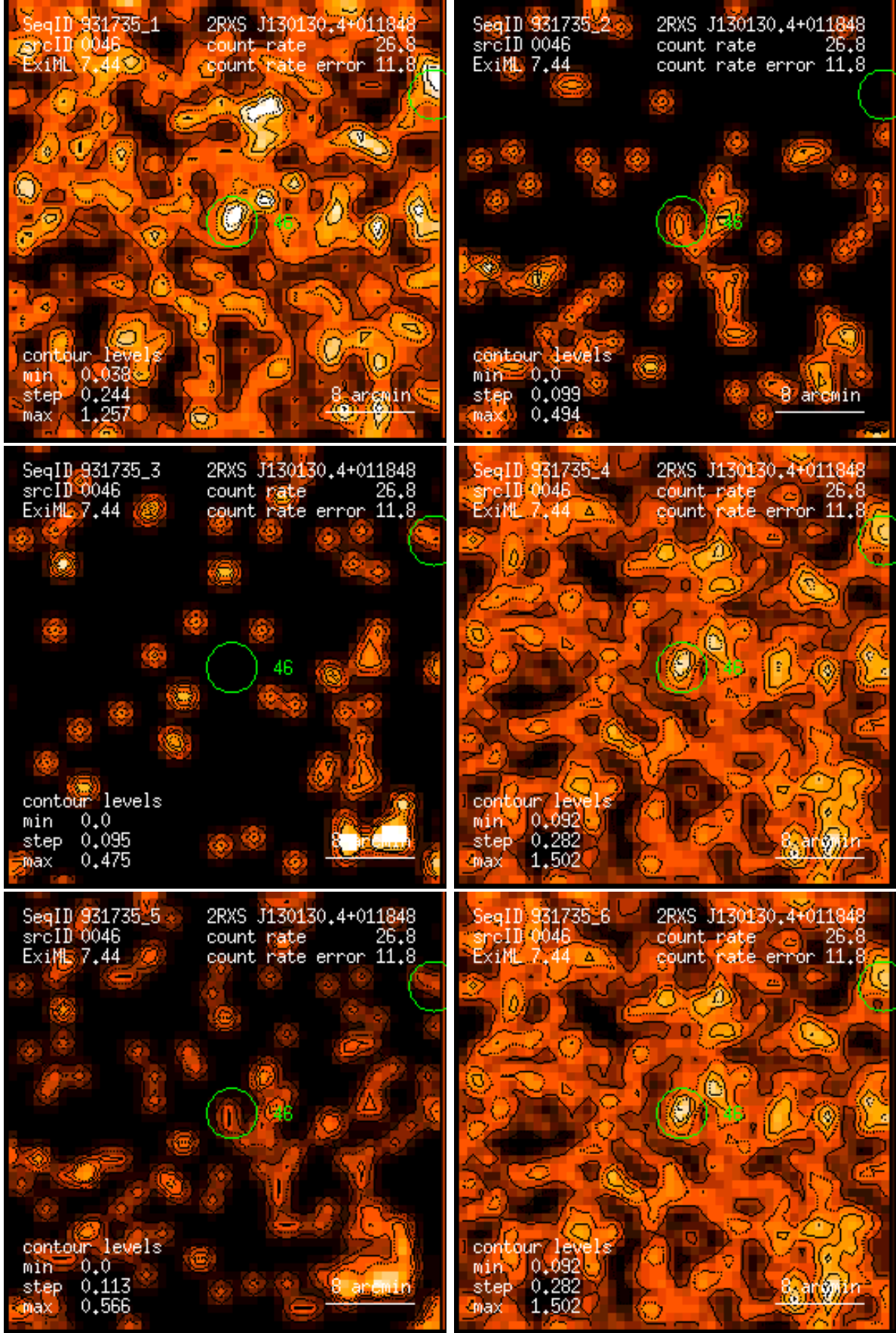
Figure 46: RASS 931735: detection 0046: band rate images, Gaussian filter: (1) PSPC channels 11 – 41, (2) 52 – 90, (3) 91 – 201, (4) 11 – 235, (5) 52 – 201, (6) 11 – 201. Broad band rates in counts/ks. Band rate contour levels in counts/ks/arcmin 2 .
