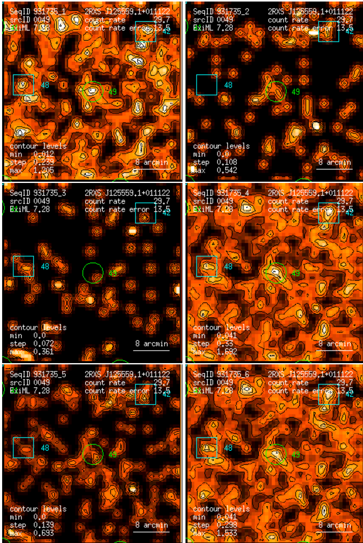
Figure 49: RASS 931735: detection 0049: band rate images, Gaussian filter: (1) PSPC channels 11 – 41, (2) 52 – 90, (3) 91 – 201, (4) 11 – 235, (5) 52 – 201, (6) 11 – 201. Broad band rates in counts/ks. Band rate contour levels in counts/ks/arcmin 2 .
