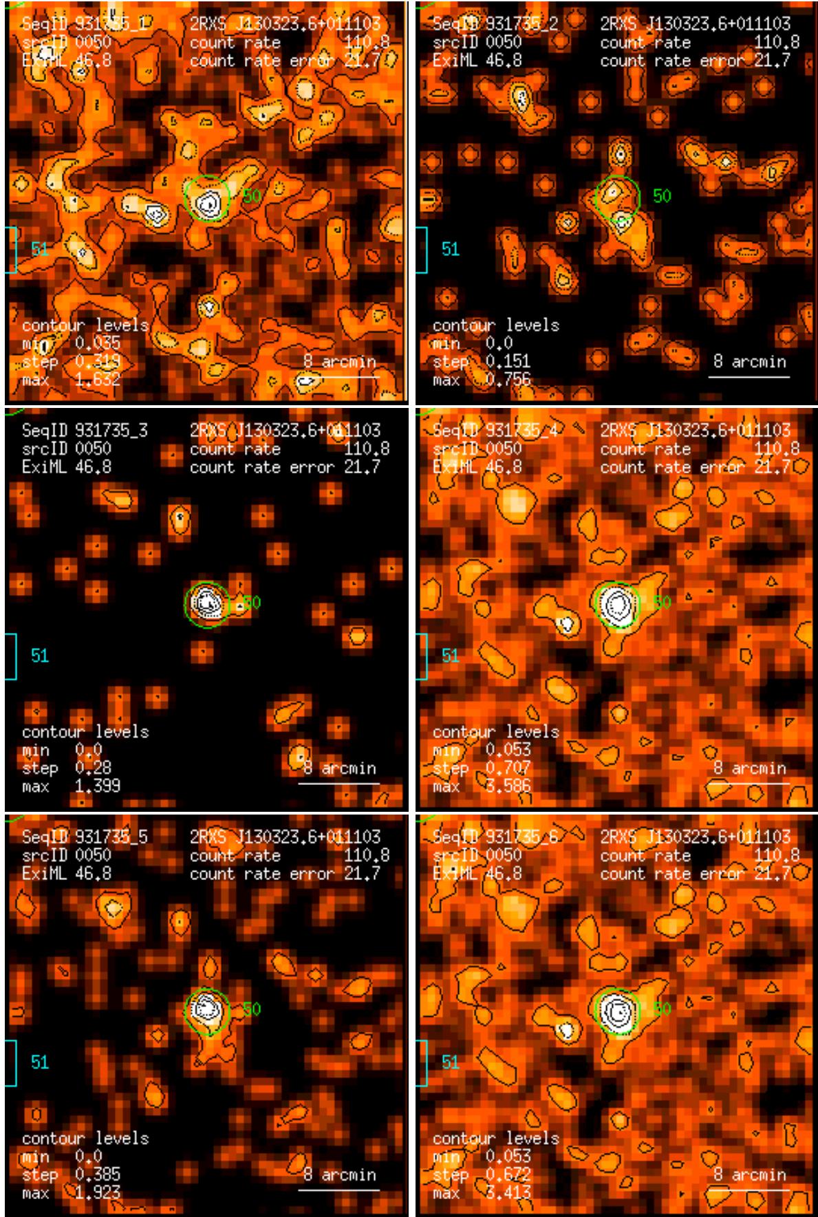
Figure 50: RASS 931735: detection 0050: band rate images, Gaussian filter: (1) PSPC channels 11 – 41, (2) 52 – 90, (3) 91 – 201, (4) 11 – 235, (5) 52 – 201, (6) 11 – 201. Broad band rates in counts/ks. Band rate contour levels in counts/ks/arcmin 2 .
