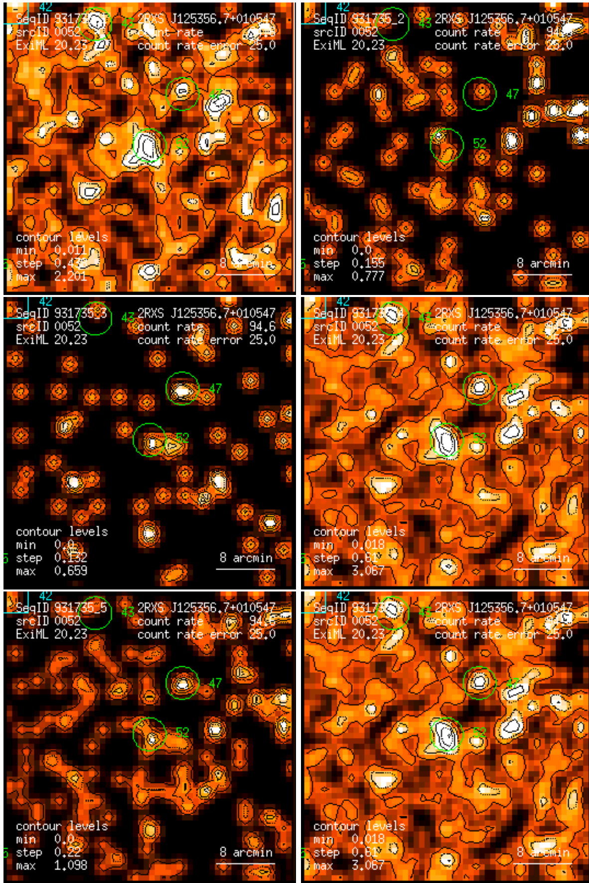
Figure 52: RASS 931735: detection 0052: band rate images, Gaussian filter: (1) PSPC channels 11 – 41, (2) 52 – 90, (3) 91 – 201, (4) 11 – 235, (5) 52 – 201, (6) 11 – 201. Broad band rates in counts/ks. Band rate contour levels in counts/ks/arcmin 2 .
