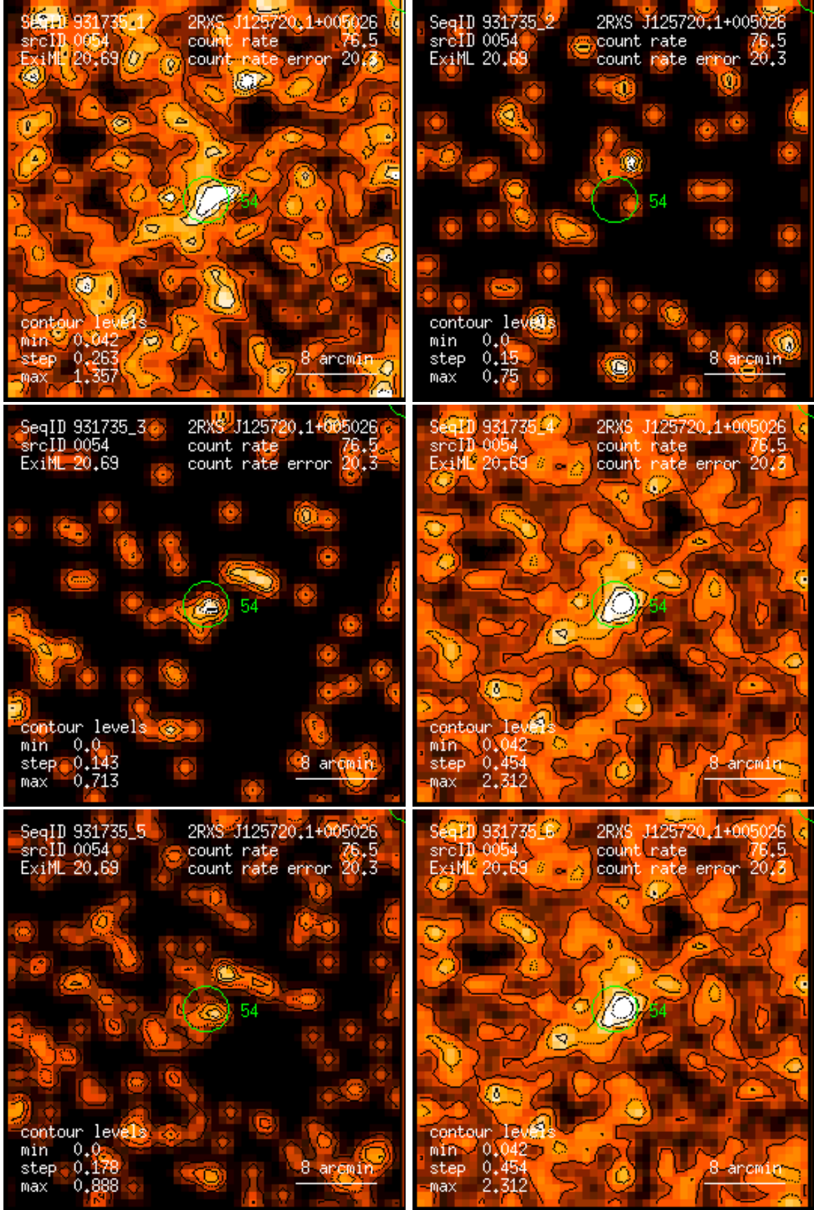
Figure 54: RASS 931735: detection 0054: band rate images, Gaussian filter: (1) PSPC channels 11 – 41, (2) 52 – 90, (3) 91 – 201, (4) 11 – 235, (5) 52 – 201, (6) 11 – 201. Broad band rates in counts/ks. Band rate contour levels in counts/ks/arcmin 2 .
