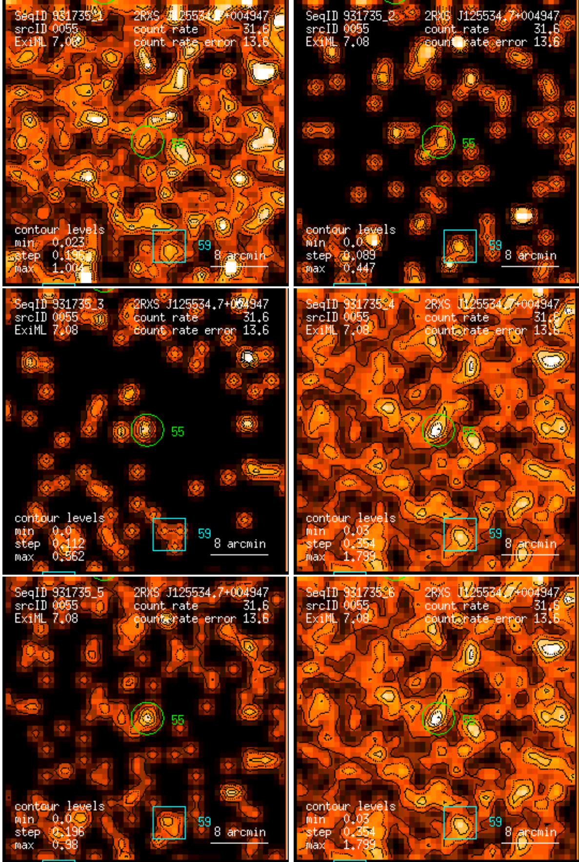
Figure 55: RASS 931735: detection 0055: band rate images, Gaussian filter: (1) PSPC channels 11 – 41, (2) 52 – 90, (3) 91 – 201, (4) 11 – 235, (5) 52 – 201, (6) 11 – 201. Broad band rates in counts/ks. Band rate contour levels in counts/ks/arcmin 2 .
