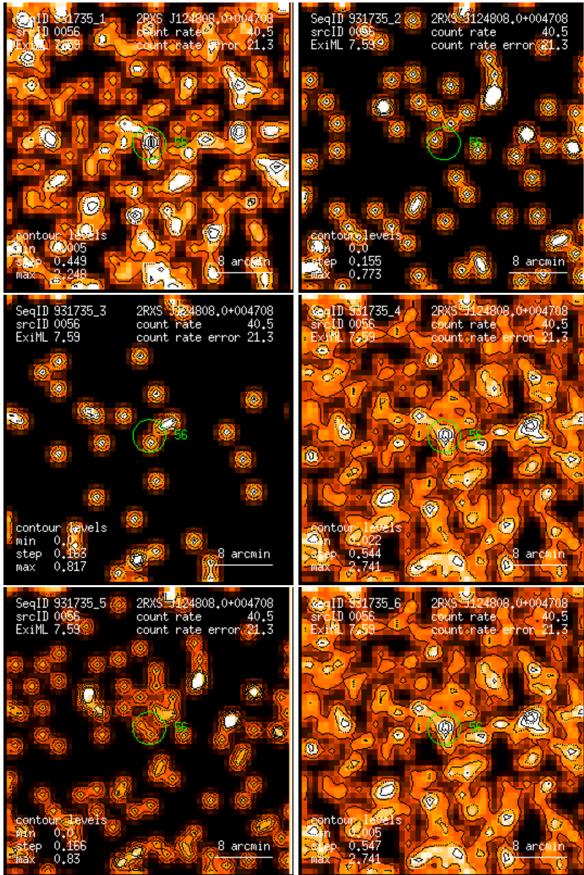
Figure 56: RASS 931735: detection 0056: band rate images, Gaussian filter: (1) PSPC channels 11 – 41, (2) 52 – 90, (3) 91 – 201, (4) 11 – 235, (5) 52 – 201, (6) 11 – 201. Broad band rates in counts/ks. Band rate contour levels in counts/ks/arcmin 2 .
