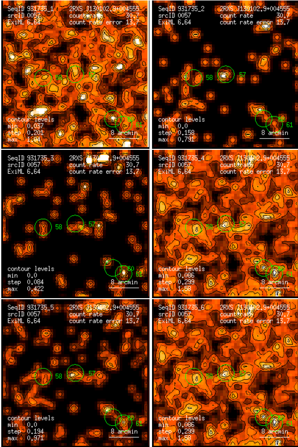
Figure 57: RASS 931735: detection 0057: band rate images, Gaussian filter: (1) PSPC channels 11 – 41, (2) 52 – 90, (3) 91 – 201, (4) 11 – 235, (5) 52 – 201, (6) 11 – 201. Broad band rates in counts/ks. Band rate contour levels in counts/ks/arcmin 2 .
