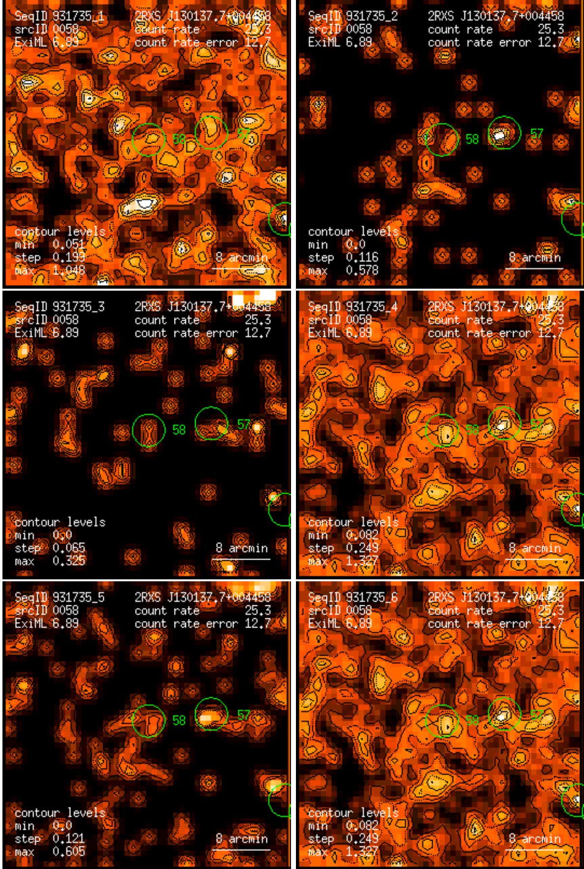
Figure 58: RASS 931735: detection 0058: band rate images, Gaussian filter: (1) PSPC channels 11 – 41, (2) 52 – 90, (3) 91 – 201, (4) 11 – 235, (5) 52 – 201, (6) 11 – 201. Broad band rates in counts/ks. Band rate contour levels in counts/ks/arcmin 2 .
