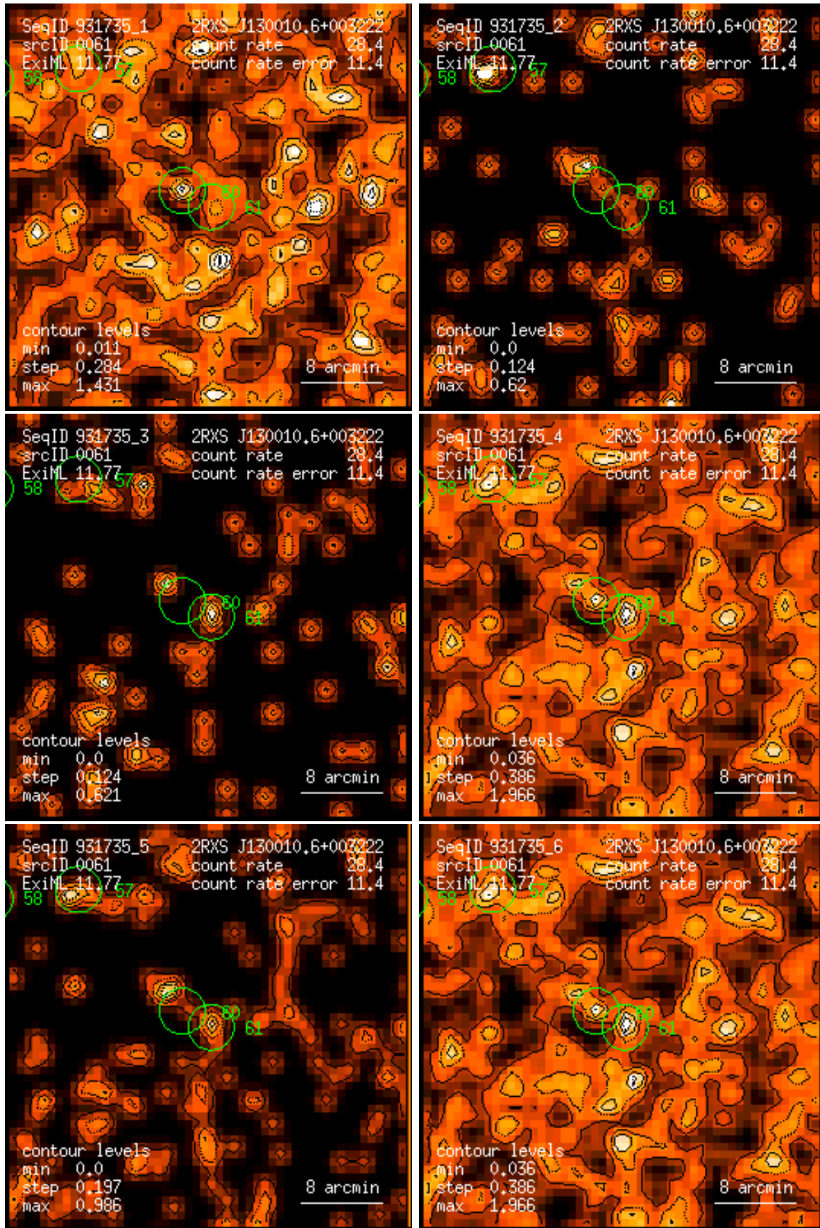
Figure 61: RASS 931735: detection 0061: band rate images, Gaussian filter: (1) PSPC channels 11 – 41, (2) 52 – 90, (3) 91 – 201, (4) 11 – 235, (5) 52 – 201, (6) 11 – 201. Broad band rates in counts/ks. Band rate contour levels in counts/ks/arcmin 2 .
