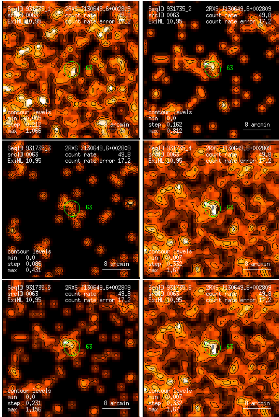
Figure 63: RASS 931735: detection 0063: band rate images, Gaussian filter: (1) PSPC channels 11 – 41, (2) 52 – 90, (3) 91 – 201, (4) 11 – 235, (5) 52 – 201, (6) 11 – 201. Broad band rates in counts/ks. Band rate contour levels in counts/ks/arcmin 2 .
