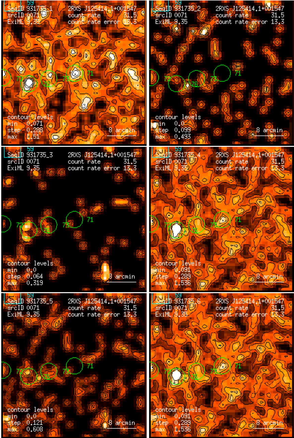
Figure 71: RASS 931735: detection 0071: band rate images, Gaussian filter: (1) PSPC channels 11 – 41, (2) 52 – 90, (3) 91 – 201, (4) 11 – 235, (5) 52 – 201, (6) 11 – 201. Broad band rates in counts/ks. Band rate contour levels in counts/ks/arcmin 2 .
