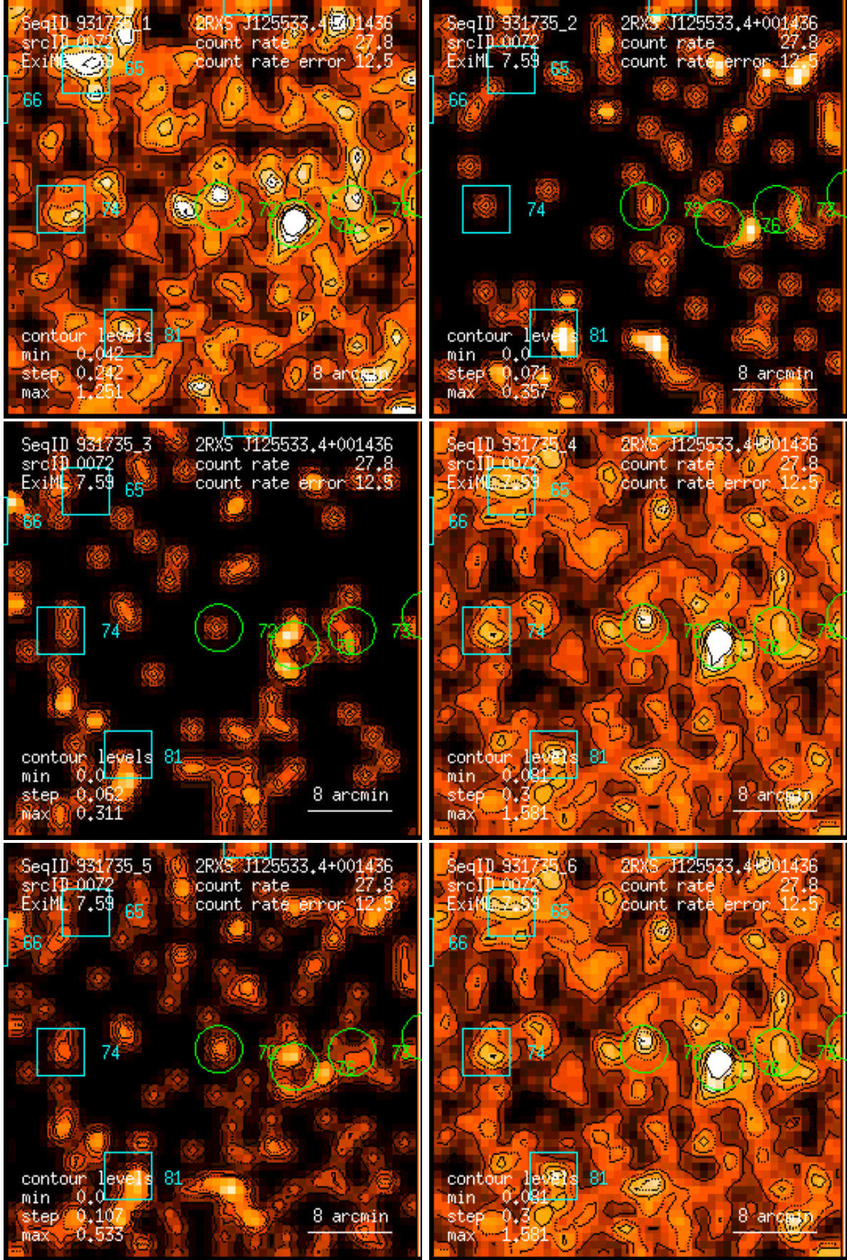
Figure 72: RASS 931735: detection 0072: band rate images, Gaussian filter: (1) PSPC channels 11 – 41, (2) 52 – 90, (3) 91 – 201, (4) 11 – 235, (5) 52 – 201, (6) 11 – 201. Broad band rates in counts/ks. Band rate contour levels in counts/ks/arcmin 2 .
