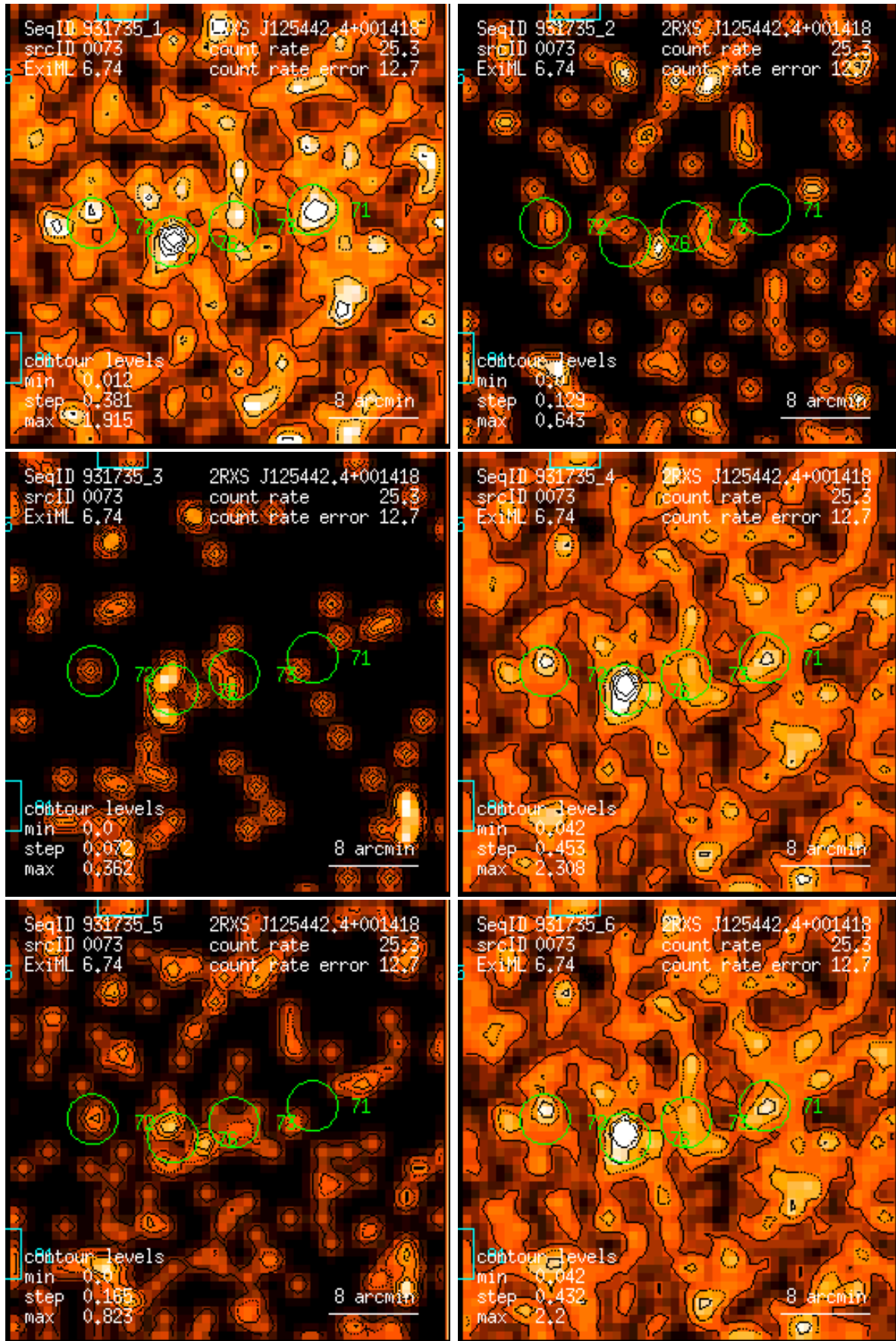
Figure 73: RASS 931735: detection 0073: band rate images, Gaussian filter: (1) PSPC channels 11 – 41, (2) 52 – 90, (3) 91 – 201, (4) 11 – 235, (5) 52 – 201, (6) 11 – 201. Broad band rates in counts/ks. Band rate contour levels in counts/ks/arcmin 2 .
