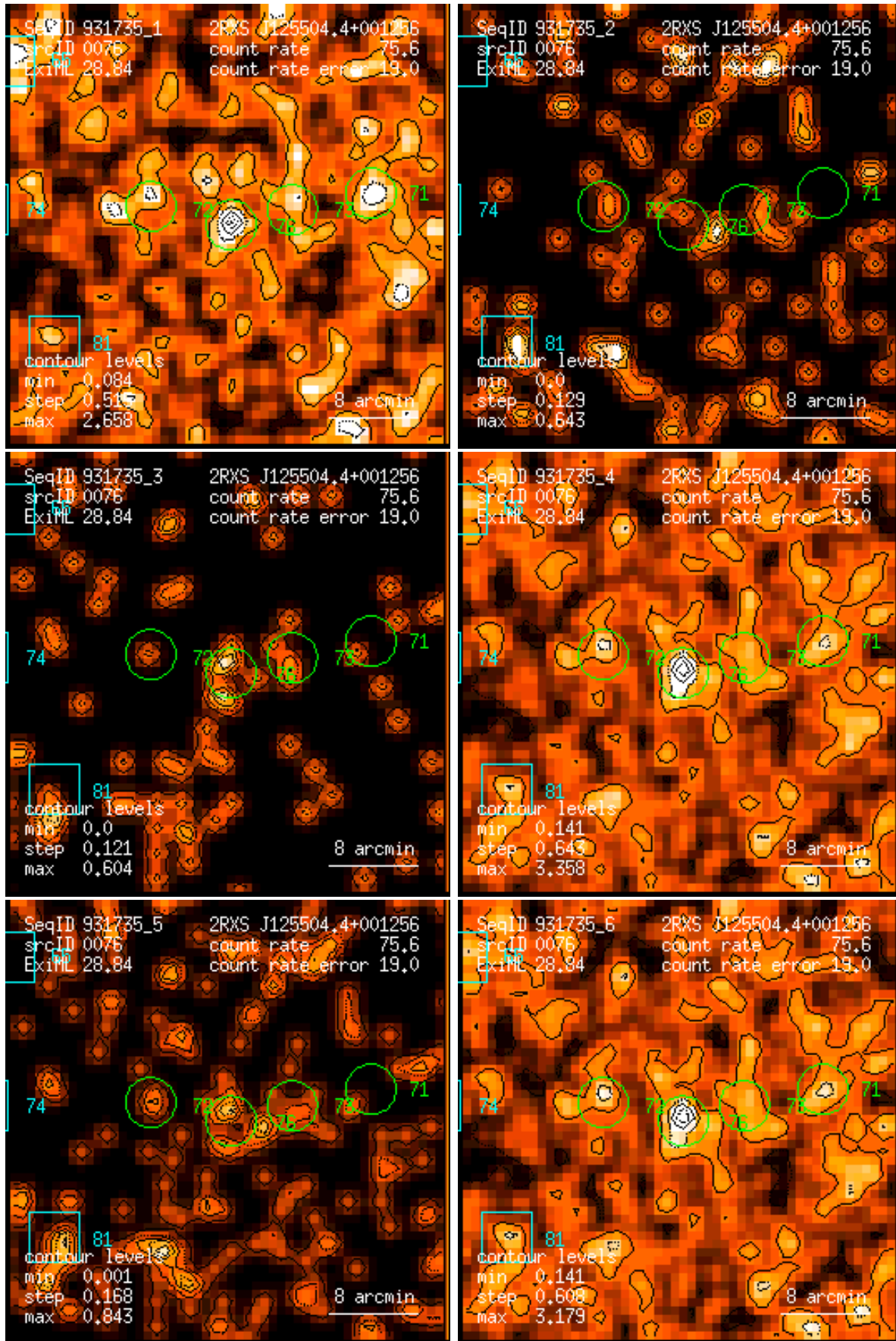
Figure 76: RASS 931735: detection 0076: band rate images, Gaussian filter: (1) PSPC channels 11 – 41, (2) 52 – 90, (3) 91 – 201, (4) 11 – 235, (5) 52 – 201, (6) 11 – 201. Broad band rates in counts/ks. Band rate contour levels in counts/ks/arcmin 2 .
