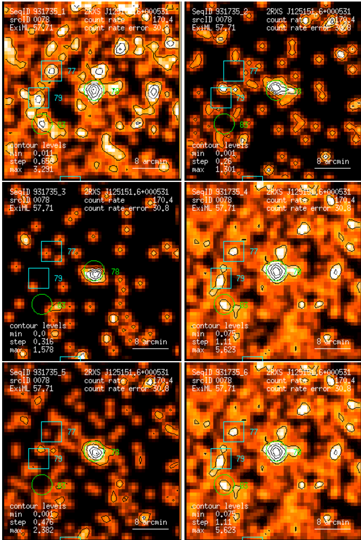
Figure 78: RASS 931735: detection 0078: band rate images, Gaussian filter: (1) PSPC channels 11 – 41, (2) 52 – 90, (3) 91 – 201, (4) 11 – 235, (5) 52 – 201, (6) 11 – 201. Broad band rates in counts/ks. Band rate contour levels in counts/ks/arcmin 2 .
