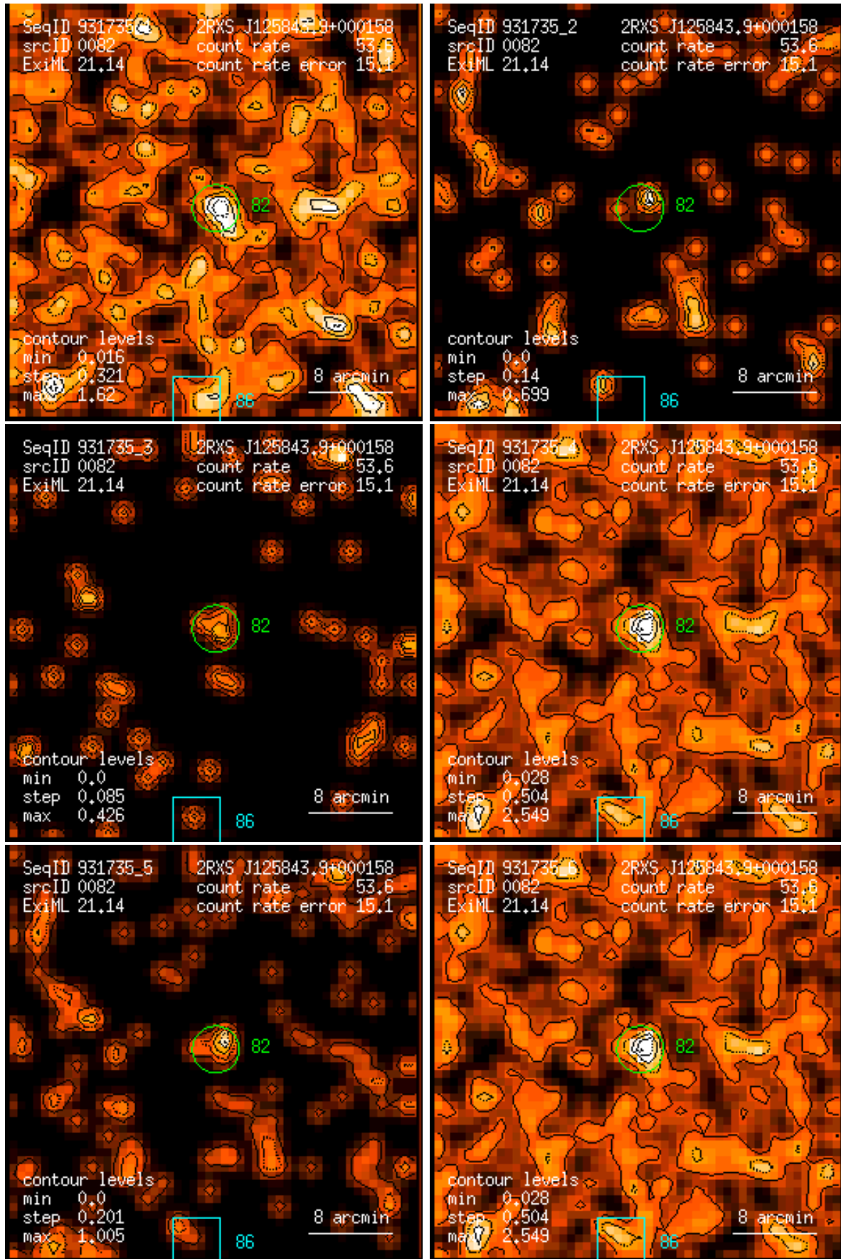
Figure 82: RASS 931735: detection 0082: band rate images, Gaussian filter: (1) PSPC channels 11 – 41, (2) 52 – 90, (3) 91 – 201, (4) 11 – 235, (5) 52 – 201, (6) 11 – 201. Broad band rates in counts/ks. Band rate contour levels in counts/ks/arcmin 2 .
