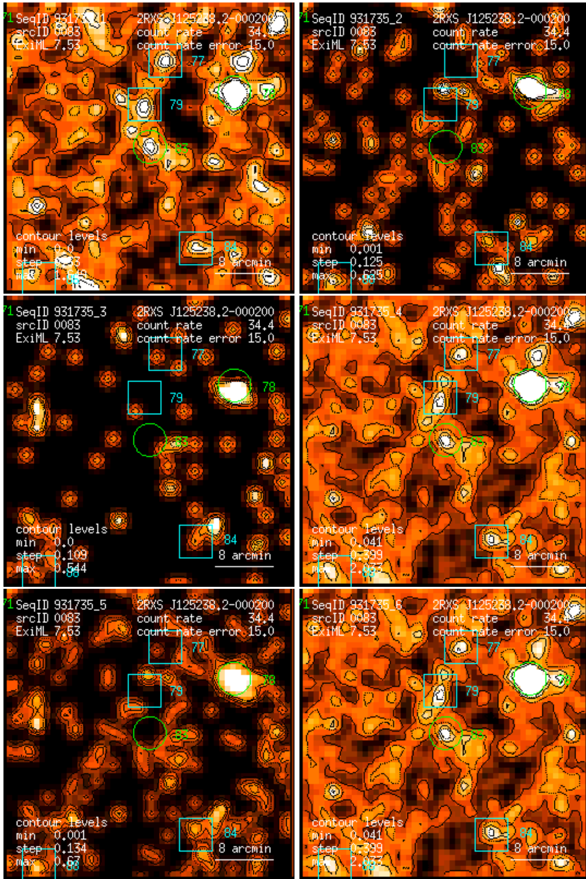
Figure 83: RASS 931735: detection 0083: band rate images, Gaussian filter: (1) PSPC channels 11 – 41, (2) 52 – 90, (3) 91 – 201, (4) 11 – 235, (5) 52 – 201, (6) 11 – 201. Broad band rates in counts/ks. Band rate contour levels in counts/ks/arcmin 2 .
