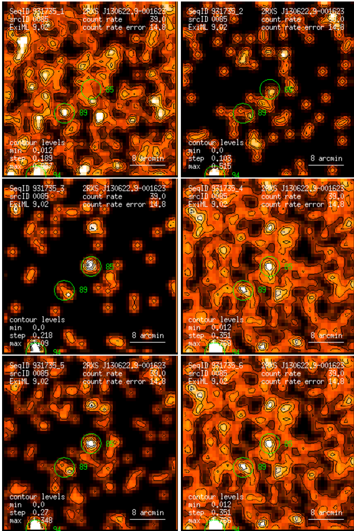
Figure 85: RASS 931735: detection 0085: band rate images, Gaussian filter: (1) PSPC channels 11 – 41, (2) 52 – 90, (3) 91 – 201, (4) 11 – 235, (5) 52 – 201, (6) 11 – 201. Broad band rates in counts/ks. Band rate contour levels in counts/ks/arcmin 2 .
