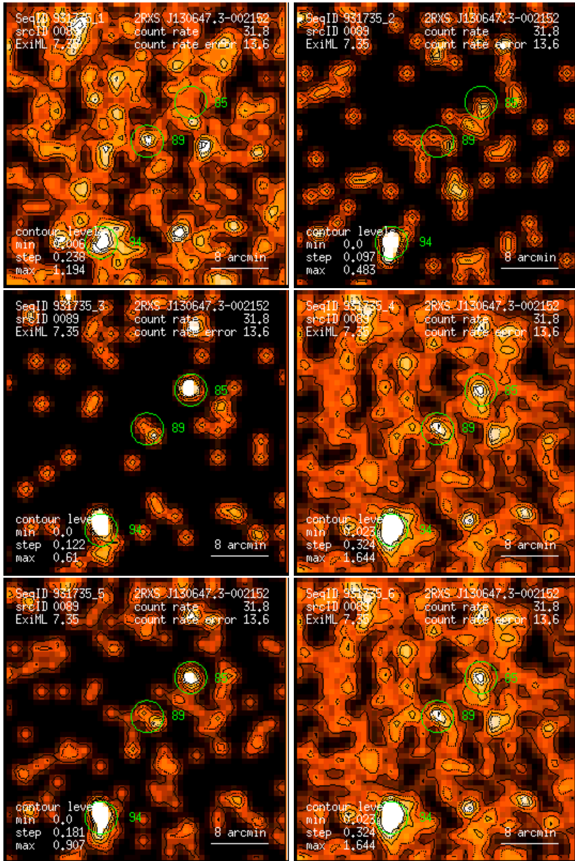
Figure 89: RASS 931735: detection 0089: band rate images, Gaussian filter: (1) PSPC channels 11 – 41, (2) 52 – 90, (3) 91 – 201, (4) 11 – 235, (5) 52 – 201, (6) 11 – 201. Broad band rates in counts/ks. Band rate contour levels in counts/ks/arcmin 2 .
