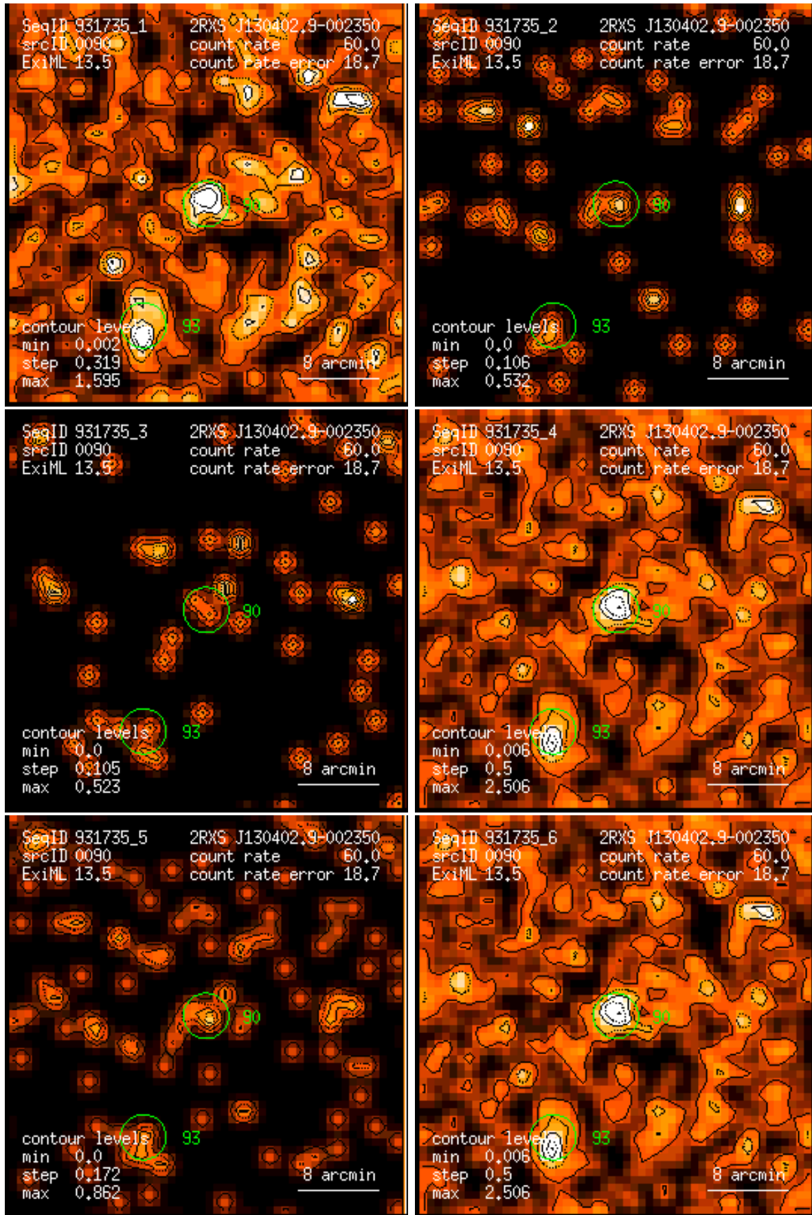
Figure 90: RASS 931735: detection 0090: band rate images, Gaussian filter: (1) PSPC channels 11 – 41, (2) 52 – 90, (3) 91 – 201, (4) 11 – 235, (5) 52 – 201, (6) 11 – 201. Broad band rates in counts/ks. Band rate contour levels in counts/ks/arcmin 2 .
