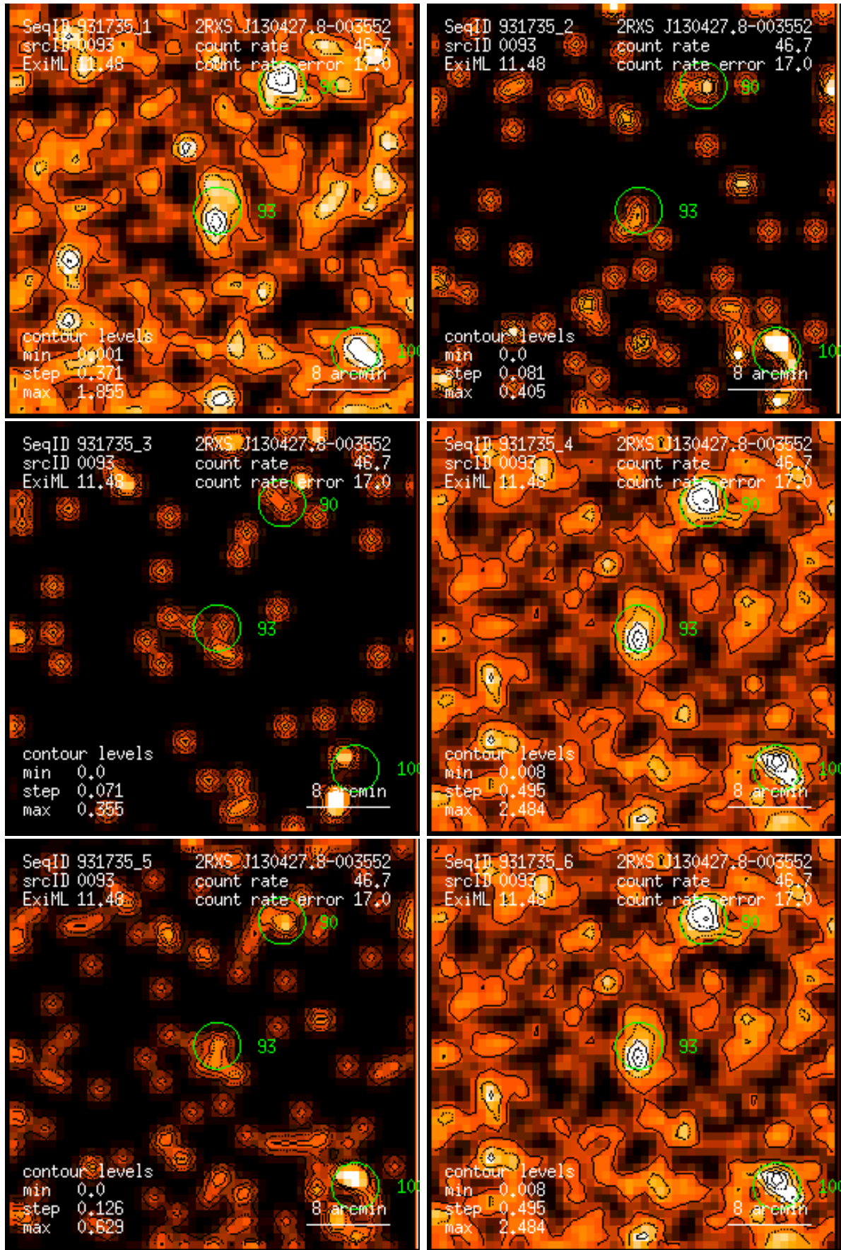
Figure 93: RASS 931735: detection 0093: band rate images, Gaussian filter: (1) PSPC channels 11 – 41, (2) 52 – 90, (3) 91 – 201, (4) 11 – 235, (5) 52 – 201, (6) 11 – 201. Broad band rates in counts/ks. Band rate contour levels in counts/ks/arcmin 2 .
