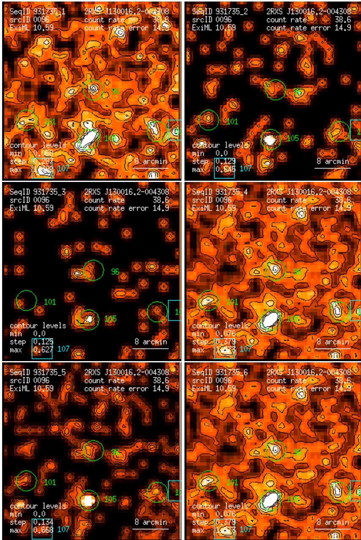
Figure 96: RASS 931735: detection 0096: band rate images, Gaussian filter: (1) PSPC channels 11 – 41, (2) 52 – 90, (3) 91 – 201, (4) 11 – 235, (5) 52 – 201, (6) 11 – 201. Broad band rates in counts/ks. Band rate contour levels in counts/ks/arcmin 2 .
