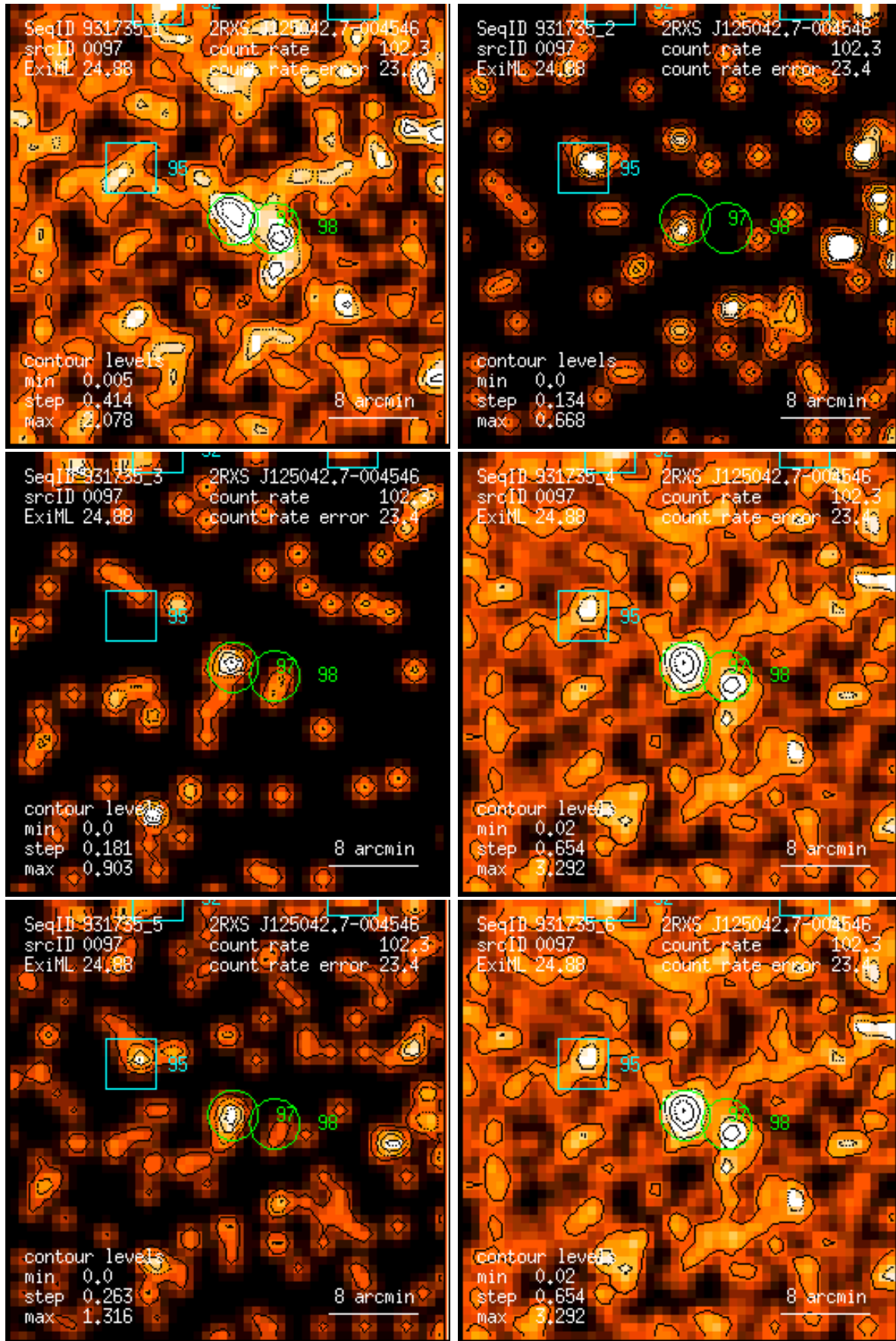
Figure 97: RASS 931735: detection 0097: band rate images, Gaussian filter: (1) PSPC channels 11 – 41, (2) 52 – 90, (3) 91 – 201, (4) 11 – 235, (5) 52 – 201, (6) 11 – 201. Broad band rates in counts/ks. Band rate contour levels in counts/ks/arcmin 2 .
