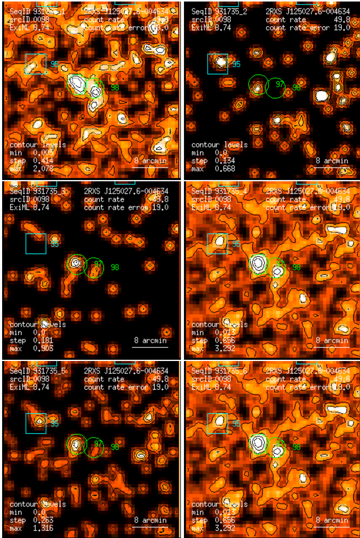
Figure 98: RASS 931735: detection 0098: band rate images, Gaussian filter: (1) PSPC channels 11 – 41, (2) 52 – 90, (3) 91 – 201, (4) 11 – 235, (5) 52 – 201, (6) 11 – 201. Broad band rates in counts/ks. Band rate contour levels in counts/ks/arcmin 2 .
