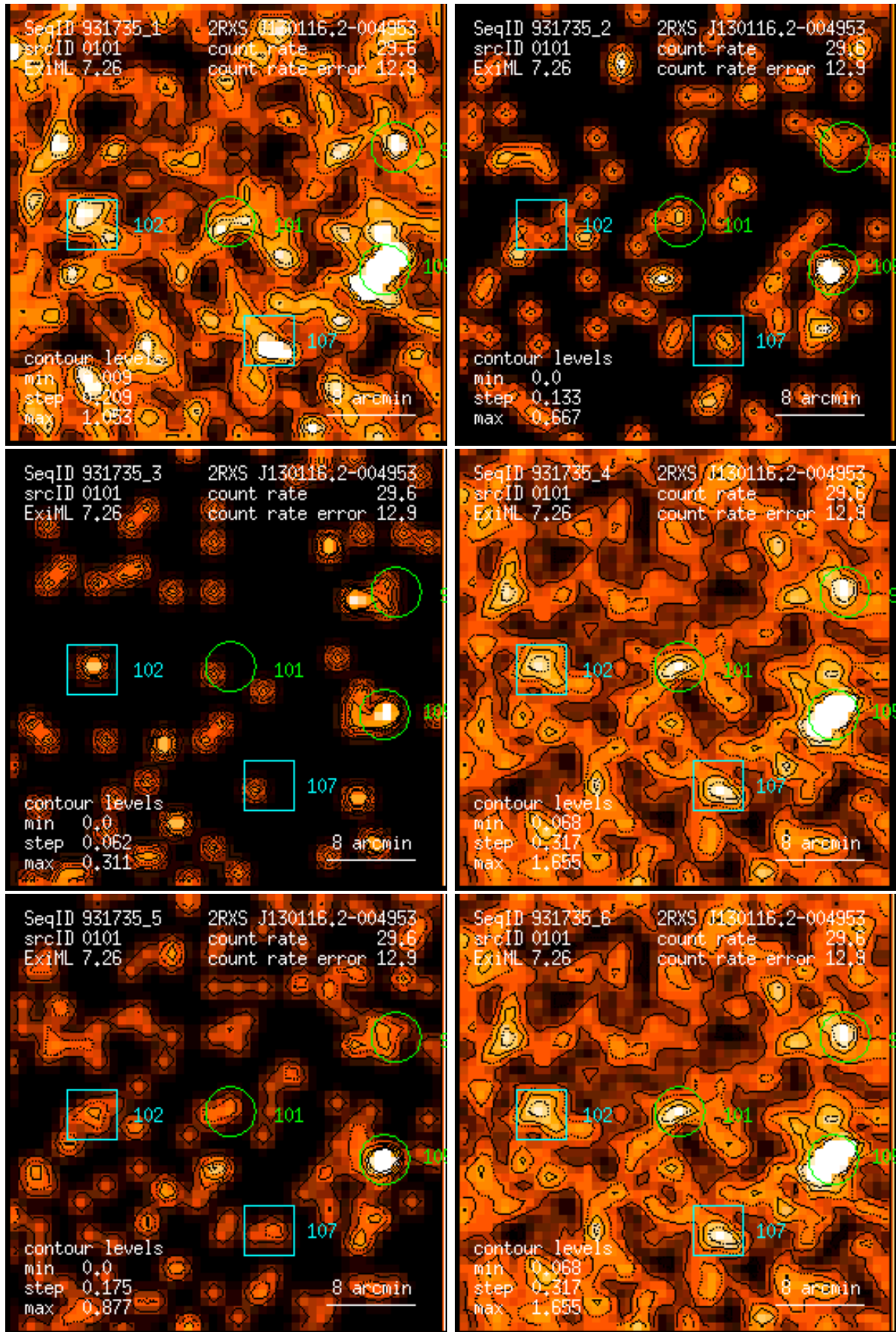
Figure 101: RASS 931735: detection 0101: band rate images, Gaussian filter: (1) PSPC channels 11 – 41, (2) 52 – 90, (3) 91 – 201, (4) 11 – 235, (5) 52 – 201, (6) 11 – 201. Broad band rates in counts/ks. Band rate contour levels in counts/ks/arcmin 2 .
