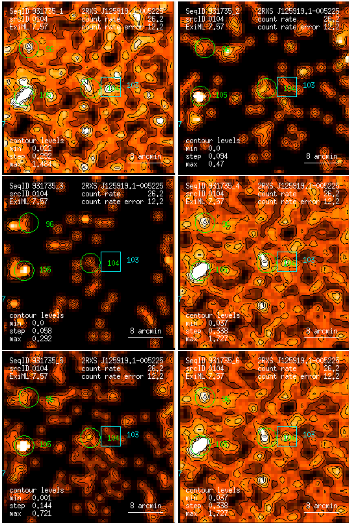
Figure 104: RASS 931735: detection 0104: band rate images, Gaussian filter: (1) PSPC channels 11 – 41, (2) 52 – 90, (3) 91 – 201, (4) 11 – 235, (5) 52 – 201, (6) 11 – 201. Broad band rates in counts/ks. Band rate contour levels in counts/ks/arcmin 2 .
