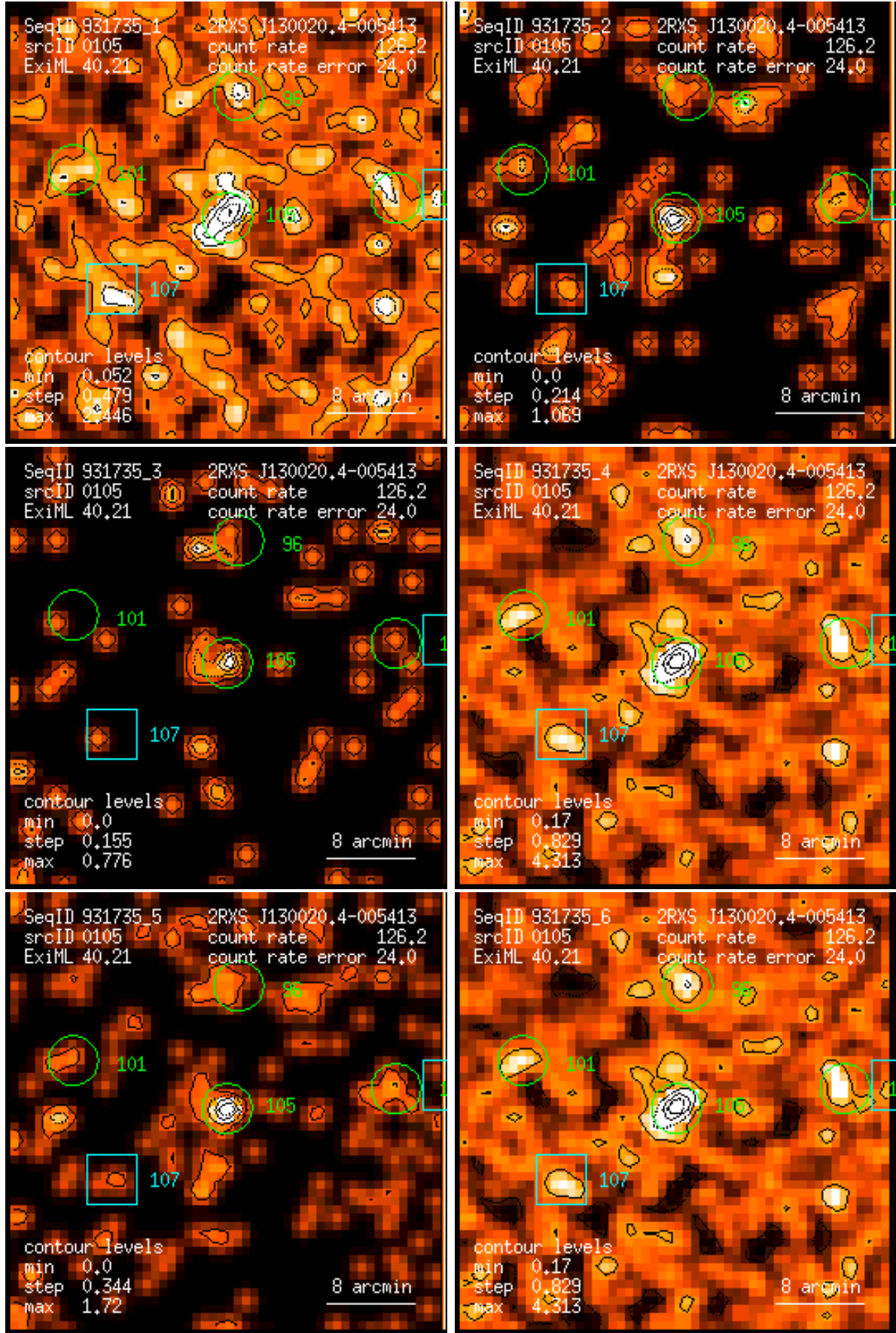
Figure 105: RASS 931735: detection 0105: band rate images, Gaussian filter: (1) PSPC channels 11 – 41, (2) 52 – 90, (3) 91 – 201, (4) 11 – 235, (5) 52 – 201, (6) 11 – 201. Broad band rates in counts/ks. Band rate contour levels in counts/ks/arcmin 2 .
