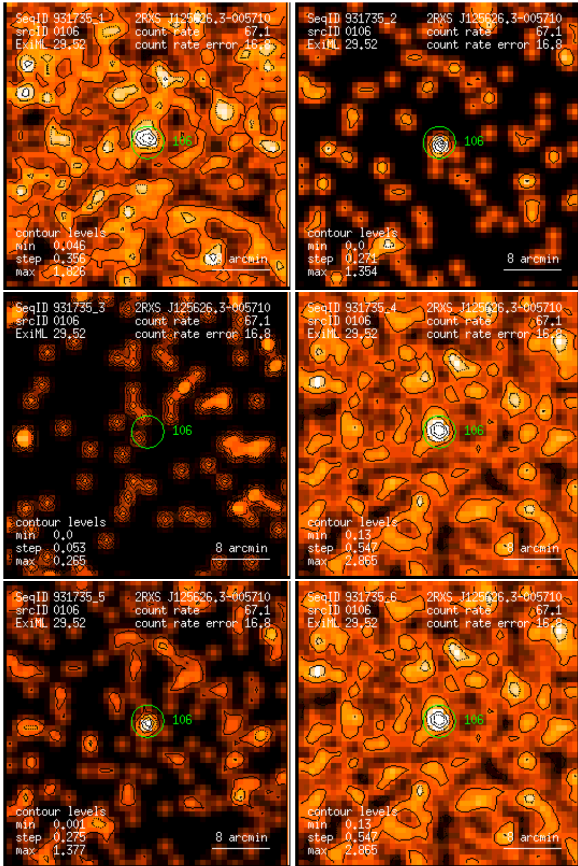
Figure 106: RASS 931735: detection 0106: band rate images, Gaussian filter: (1) PSPC channels 11 – 41, (2) 52 – 90, (3) 91 – 201, (4) 11 – 235, (5) 52 – 201, (6) 11 – 201. Broad band rates in counts/ks. Band rate contour levels in counts/ks/arcmin 2 .
