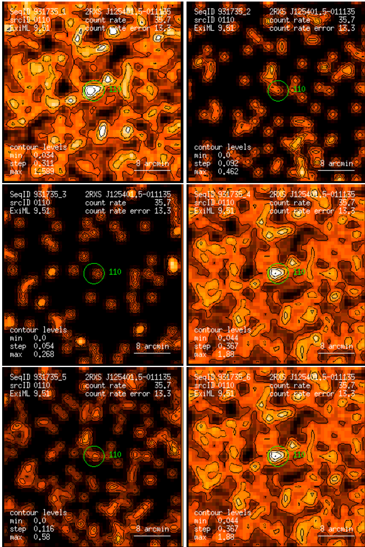
Figure 110: RASS 931735: detection 0110: band rate images, Gaussian filter: (1) PSPC channels 11 – 41, (2) 52 – 90, (3) 91 – 201, (4) 11 – 235, (5) 52 – 201, (6) 11 – 201. Broad band rates in counts/ks. Band rate contour levels in counts/ks/arcmin 2 .
