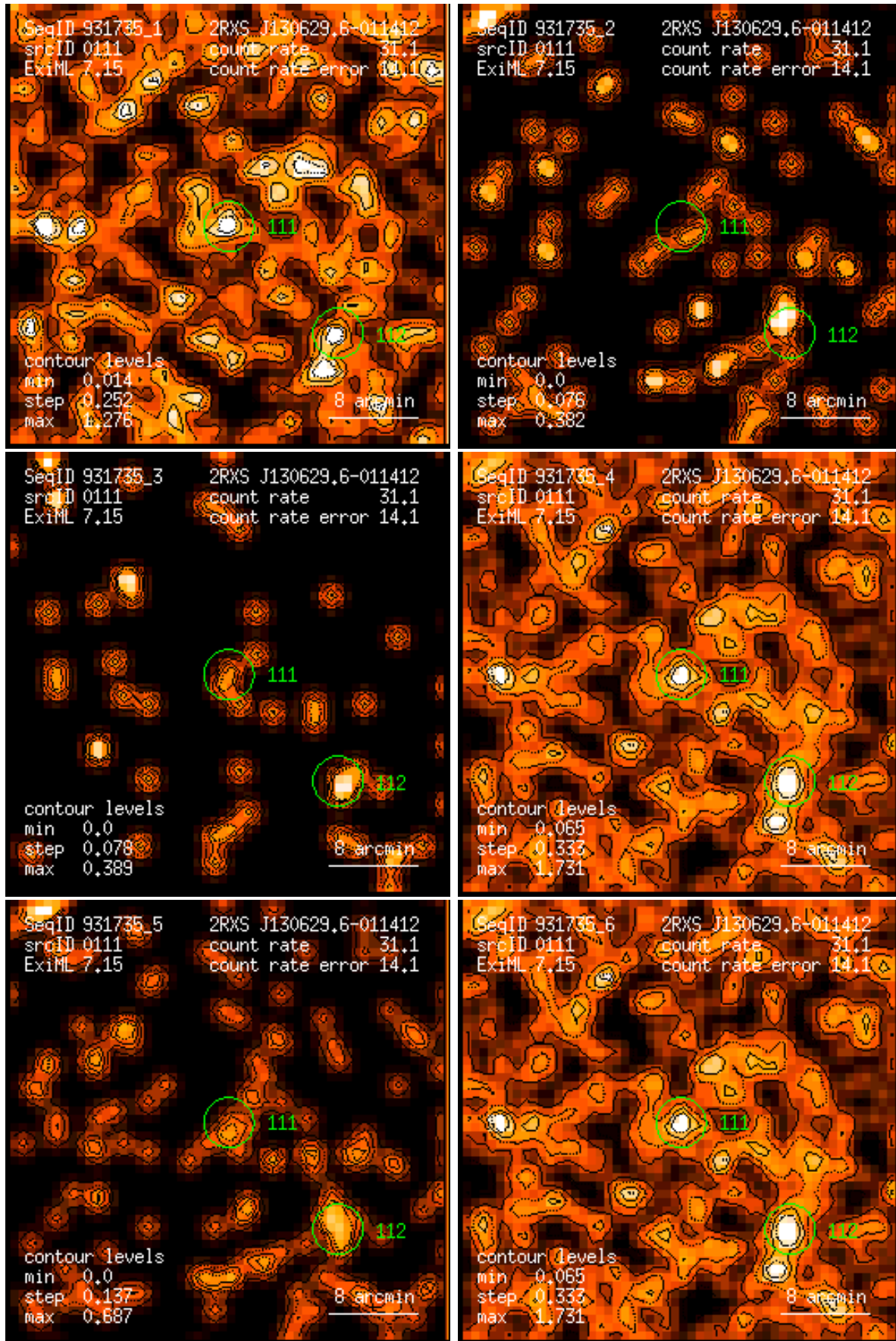
Figure 111: RASS 931735: detection 0111: band rate images, Gaussian filter: (1) PSPC channels 11 – 41, (2) 52 – 90, (3) 91 – 201, (4) 11 – 235, (5) 52 – 201, (6) 11 – 201. Broad band rates in counts/ks. Band rate contour levels in counts/ks/arcmin 2 .
