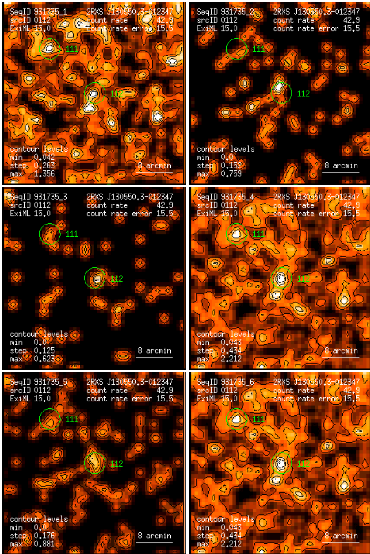
Figure 112: RASS 931735: detection 0112: band rate images, Gaussian filter: (1) PSPC channels 11 – 41, (2) 52 – 90, (3) 91 – 201, (4) 11 – 235, (5) 52 – 201, (6) 11 – 201. Broad band rates in counts/ks. Band rate contour levels in counts/ks/arcmin 2 .
