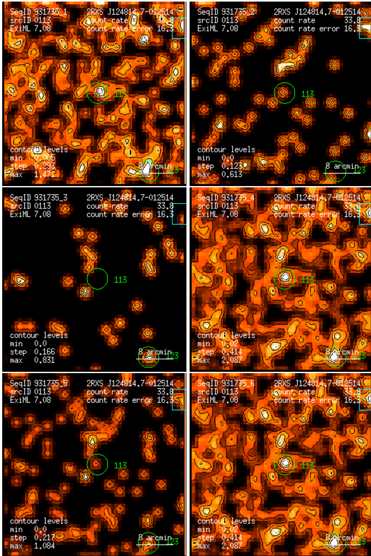
Figure 113: RASS 931735: detection 0113: band rate images, Gaussian filter: (1) PSPC channels 11 – 41, (2) 52 – 90, (3) 91 – 201, (4) 11 – 235, (5) 52 – 201, (6) 11 – 201. Broad band rates in counts/ks. Band rate contour levels in counts/ks/arcmin 2 .
