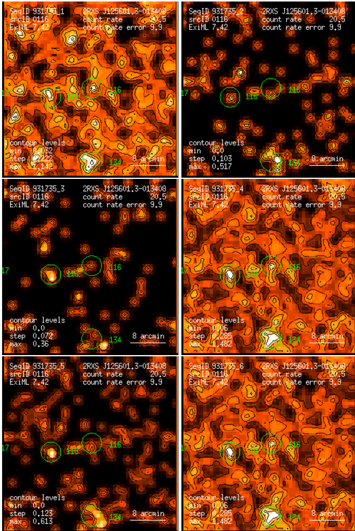
Figure 116: RASS 931735: detection 0116: band rate images, Gaussian filter: (1) PSPC channels 11 – 41, (2) 52 – 90, (3) 91 – 201, (4) 11 – 235, (5) 52 – 201, (6) 11 – 201. Broad band rates in counts/ks. Band rate contour levels in counts/ks/arcmin 2 .
