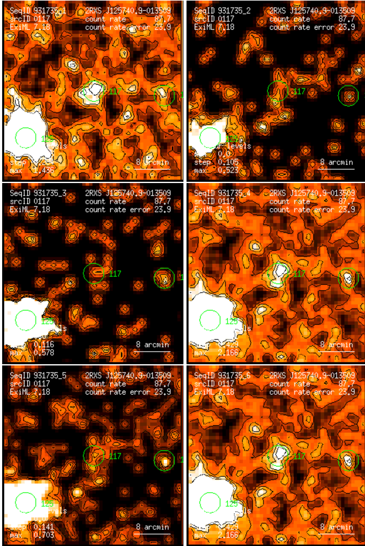
Figure 117: RASS 931735: detection 0117: band rate images, Gaussian filter: (1) PSPC channels 11 – 41, (2) 52 – 90, (3) 91 – 201, (4) 11 – 235, (5) 52 – 201, (6) 11 – 201. Broad band rates in counts/ks. Band rate contour levels in counts/ks/arcmin 2 .
