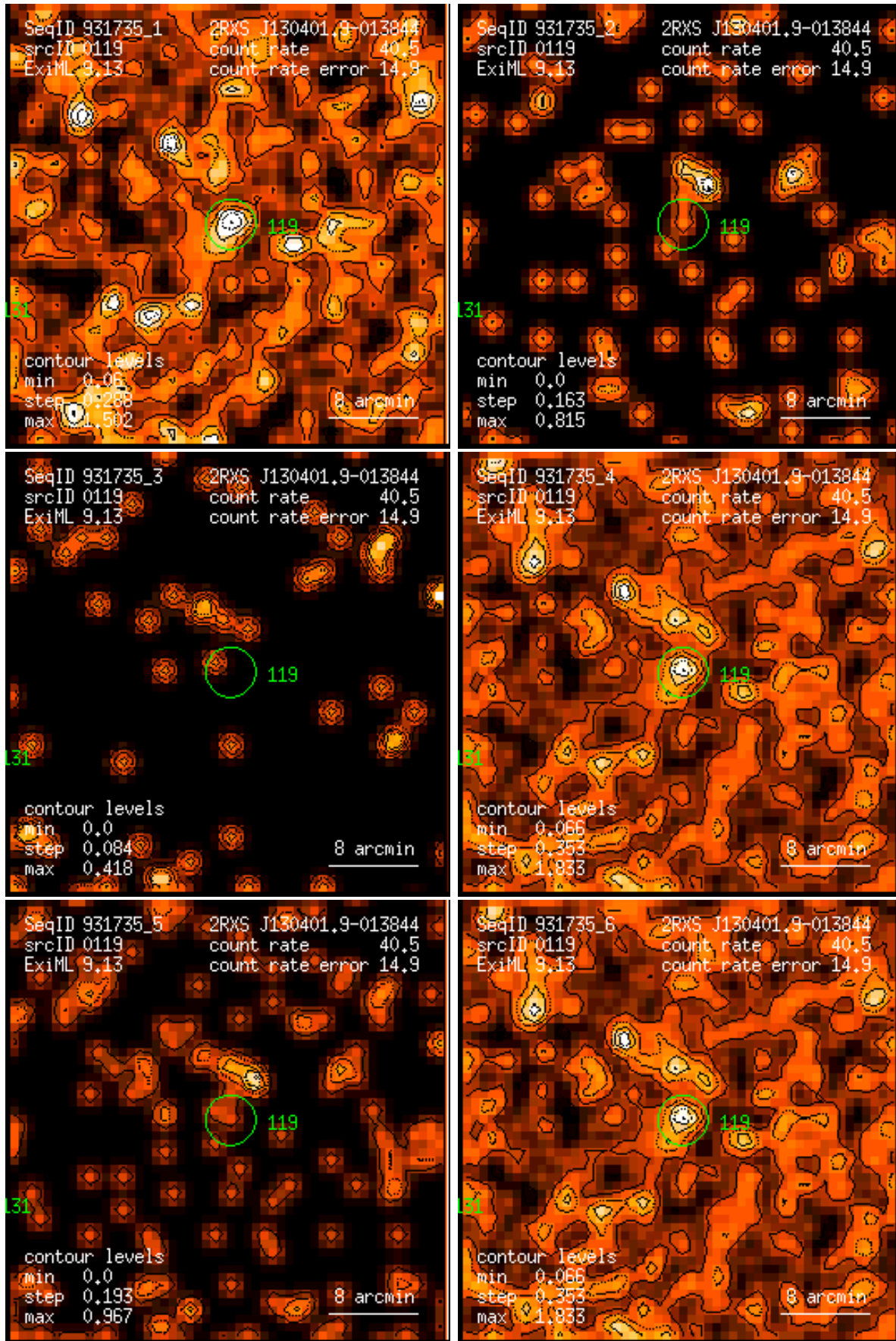
Figure 119: RASS 931735: detection 0119: band rate images, Gaussian filter: (1) PSPC channels 11 – 41, (2) 52 – 90, (3) 91 – 201, (4) 11 – 235, (5) 52 – 201, (6) 11 – 201. Broad band rates in counts/ks. Band rate contour levels in counts/ks/arcmin 2 .
