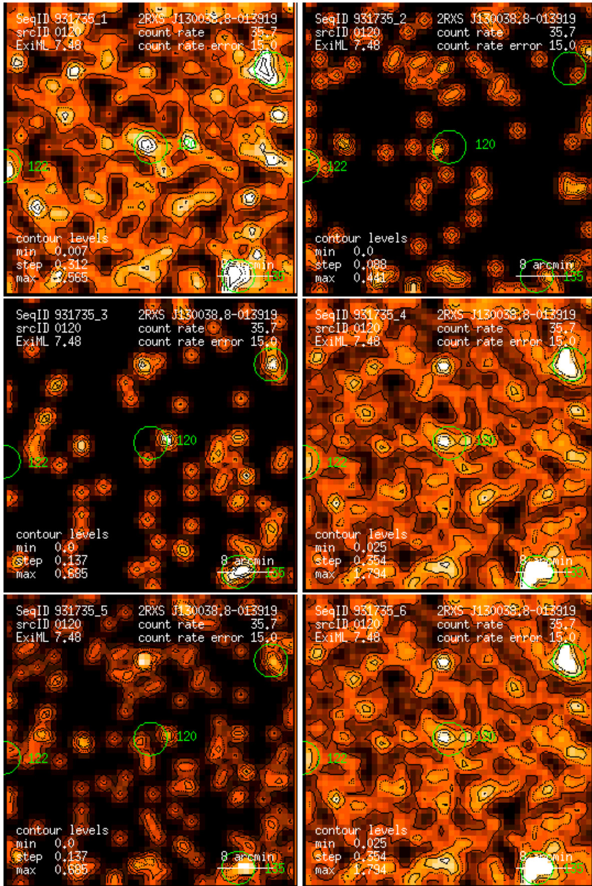
Figure 120: RASS 931735: detection 0120: band rate images, Gaussian filter: (1) PSPC channels 11 – 41, (2) 52 – 90, (3) 91 – 201, (4) 11 – 235, (5) 52 – 201, (6) 11 – 201. Broad band rates in counts/ks. Band rate contour levels in counts/ks/arcmin 2 .
