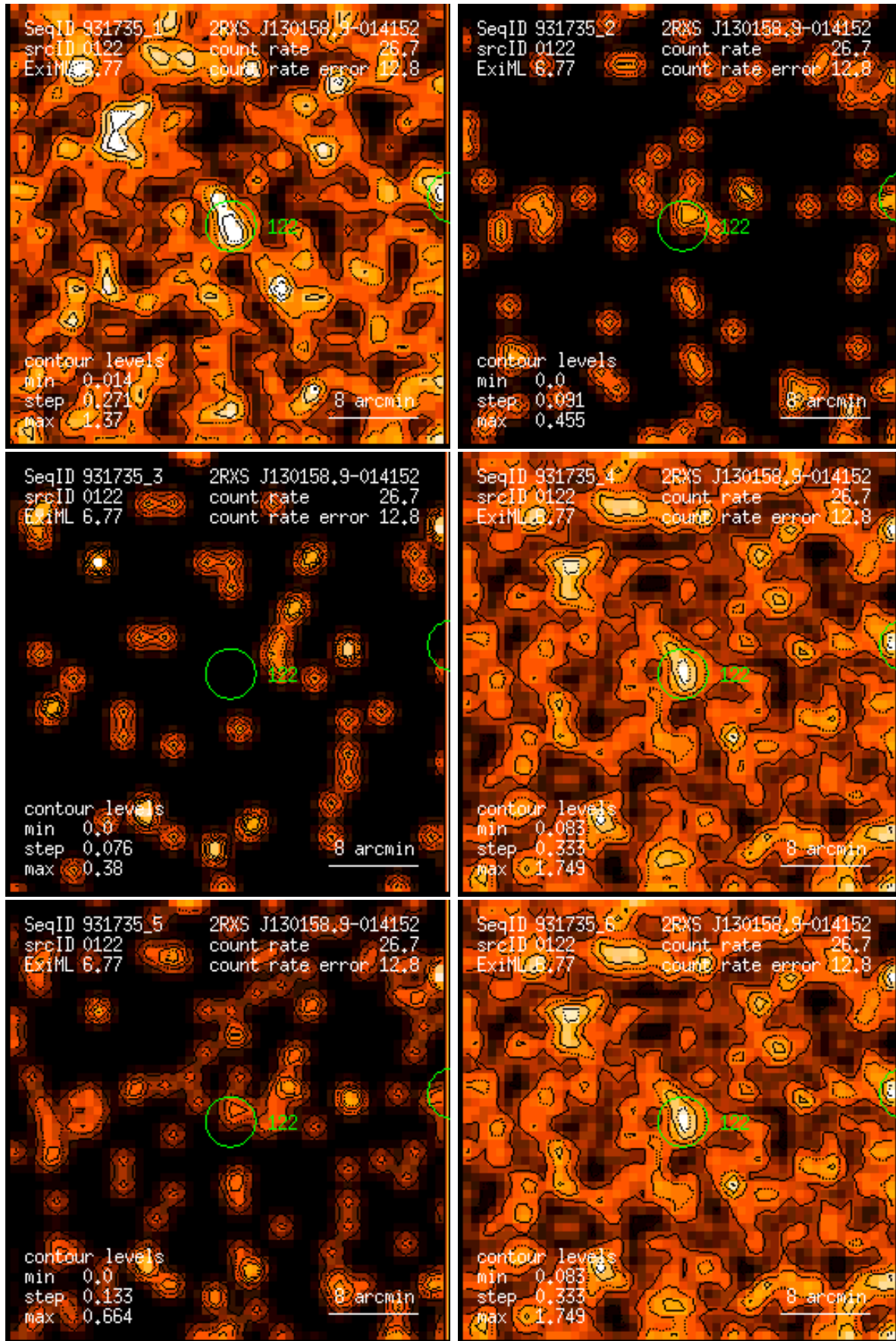
Figure 122: RASS 931735: detection 0122: band rate images, Gaussian filter: (1) PSPC channels 11 – 41, (2) 52 – 90, (3) 91 – 201, (4) 11 – 235, (5) 52 – 201, (6) 11 – 201. Broad band rates in counts/ks. Band rate contour levels in counts/ks/arcmin 2 .
