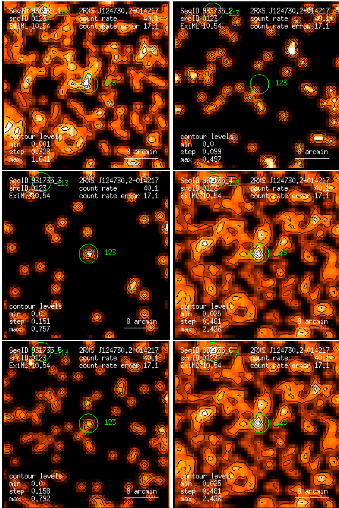
Figure 123: RASS 931735: detection 0123: band rate images, Gaussian filter: (1) PSPC channels 11 – 41, (2) 52 – 90, (3) 91 – 201, (4) 11 – 235, (5) 52 – 201, (6) 11 – 201. Broad band rates in counts/ks. Band rate contour levels in counts/ks/arcmin 2 .
