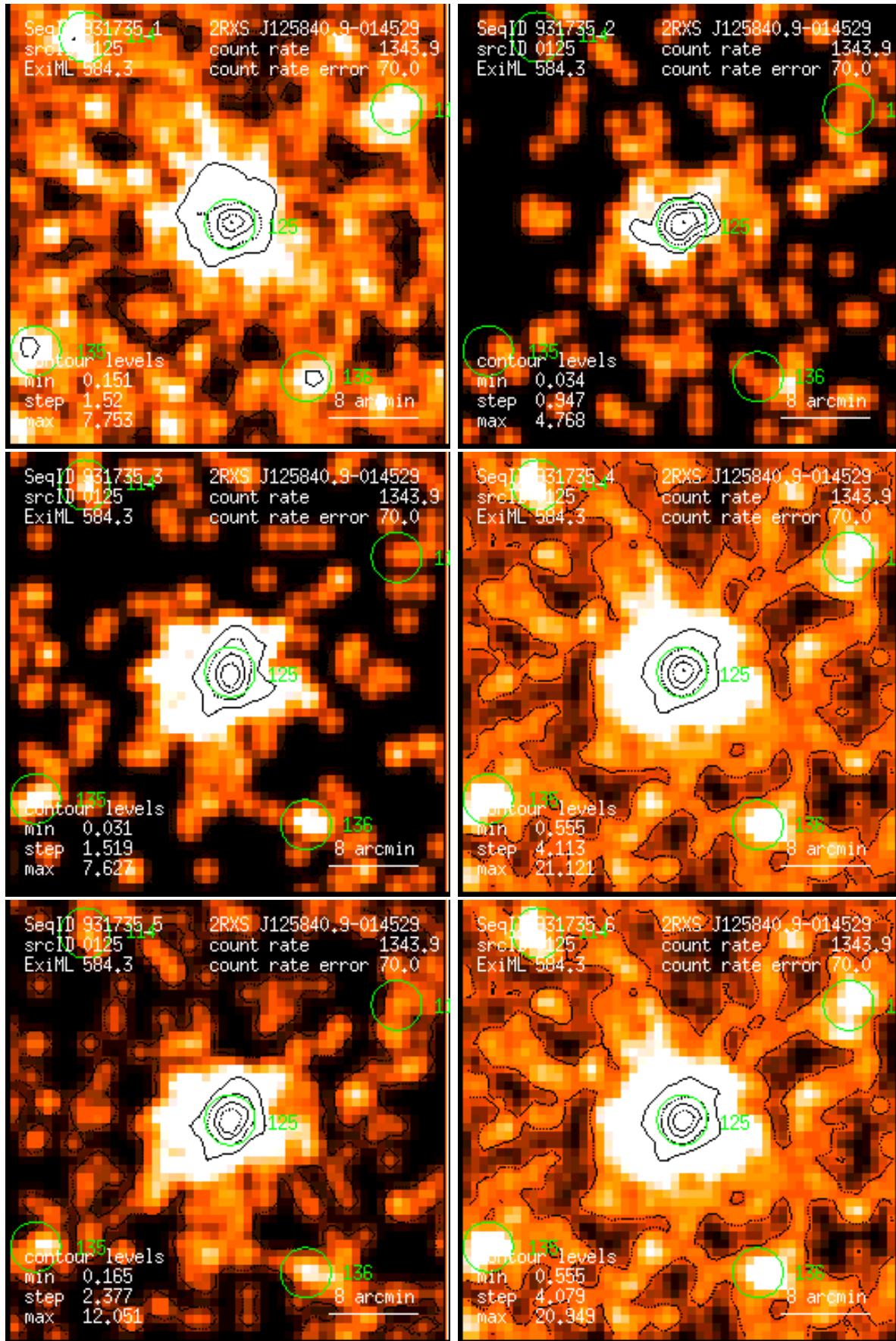
Figure 125: RASS 931735: detection 0125: band rate images, Gaussian filter: (1) PSPC channels 11 – 41, (2) 52 – 90, (3) 91 – 201, (4) 11 – 235, (5) 52 – 201, (6) 11 – 201. Broad band rates in counts/ks. Band rate contour levels in counts/ks/arcmin 2 .
