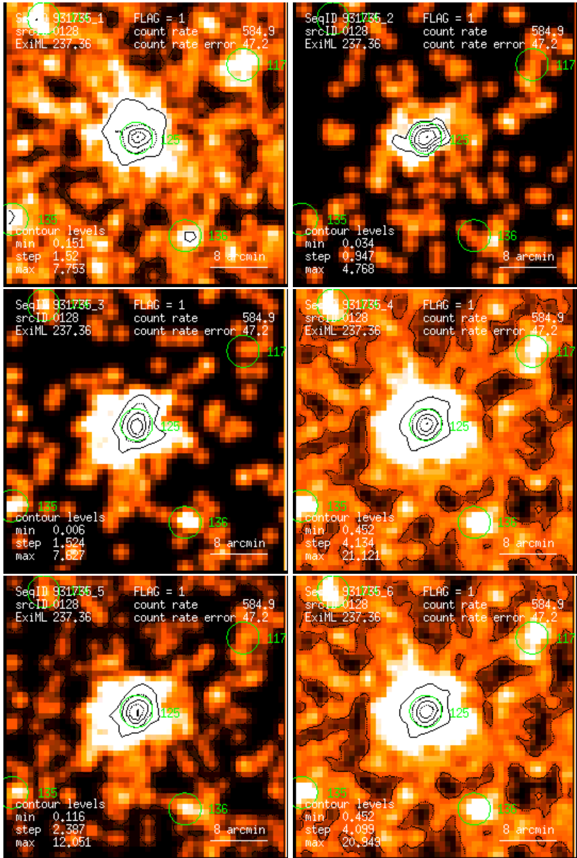
Figure 128: RASS 931735: detection 0128: band rate images, Gaussian filter: (1) PSPC channels 11 – 41, (2) 52 – 90, (3) 91 – 201, (4) 11 – 235, (5) 52 – 201, (6) 11 – 201. Broad band rates in counts/ks. Band rate contour levels in counts/ks/arcmin 2 .
