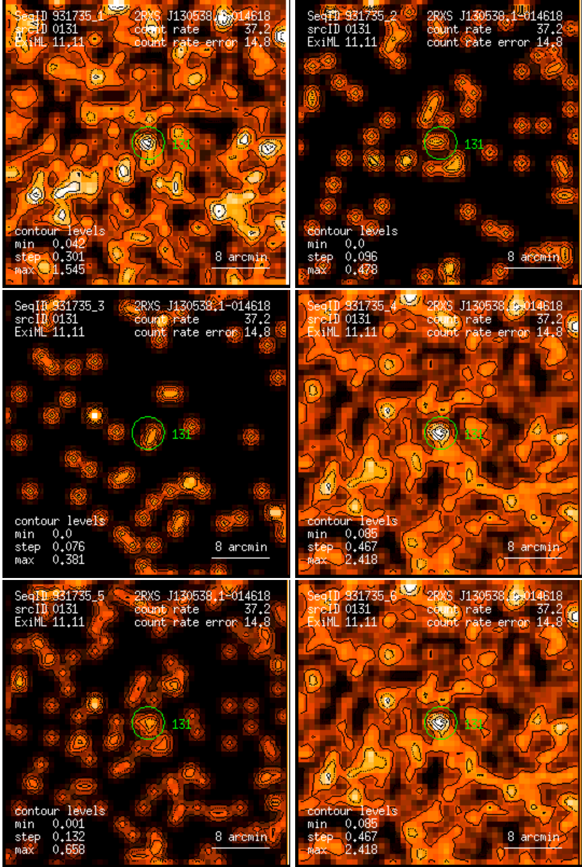
Figure 131: RASS 931735: detection 0131: band rate images, Gaussian filter: (1) PSPC channels 11 – 41, (2) 52 – 90, (3) 91 – 201, (4) 11 – 235, (5) 52 – 201, (6) 11 – 201. Broad band rates in counts/ks. Band rate contour levels in counts/ks/arcmin 2 .
