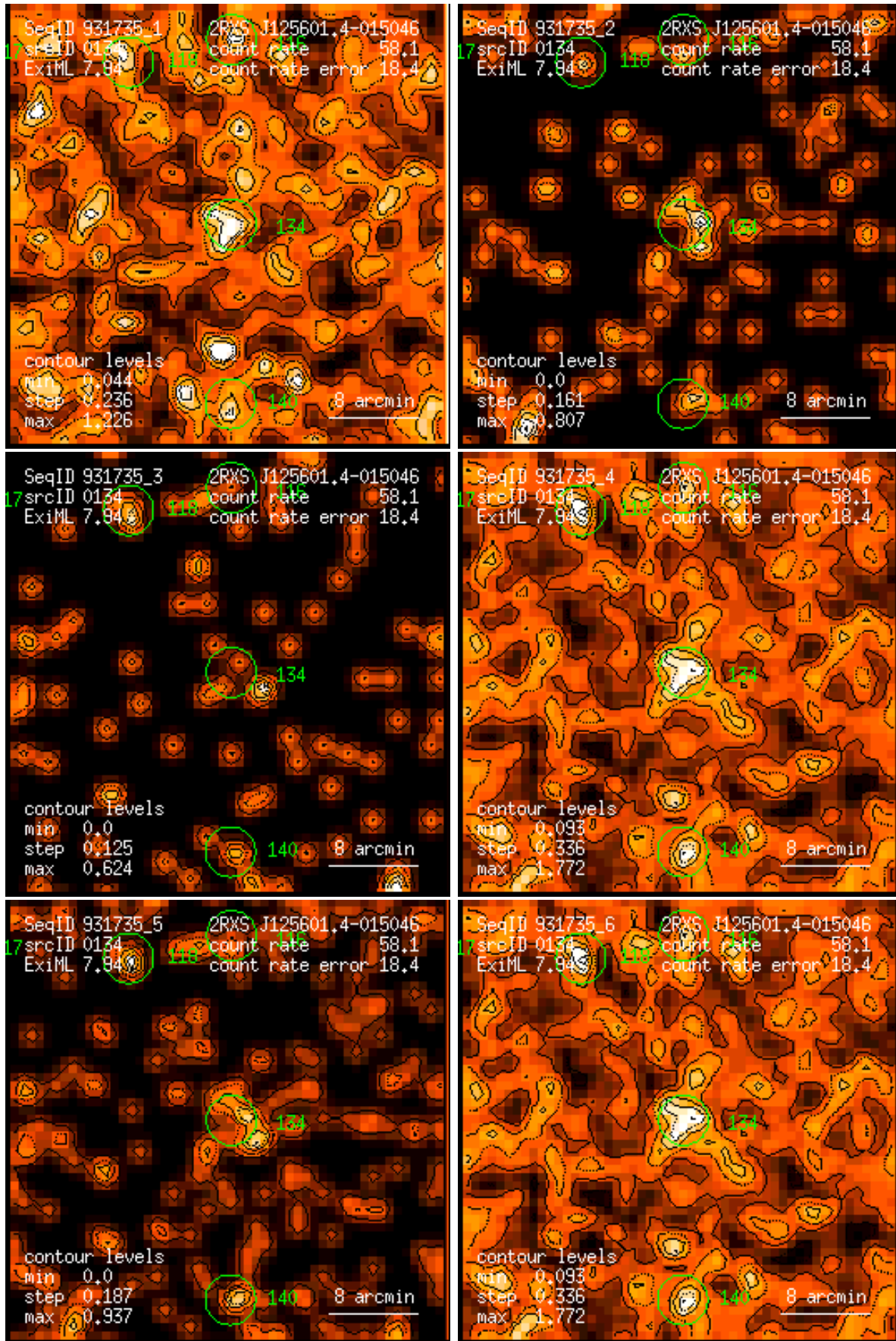
Figure 134: RASS 931735: detection 0134: band rate images, Gaussian filter: (1) PSPC channels 11 – 41, (2) 52 – 90, (3) 91 – 201, (4) 11 – 235, (5) 52 – 201, (6) 11 – 201. Broad band rates in counts/ks. Band rate contour levels in counts/ks/arcmin 2 .
