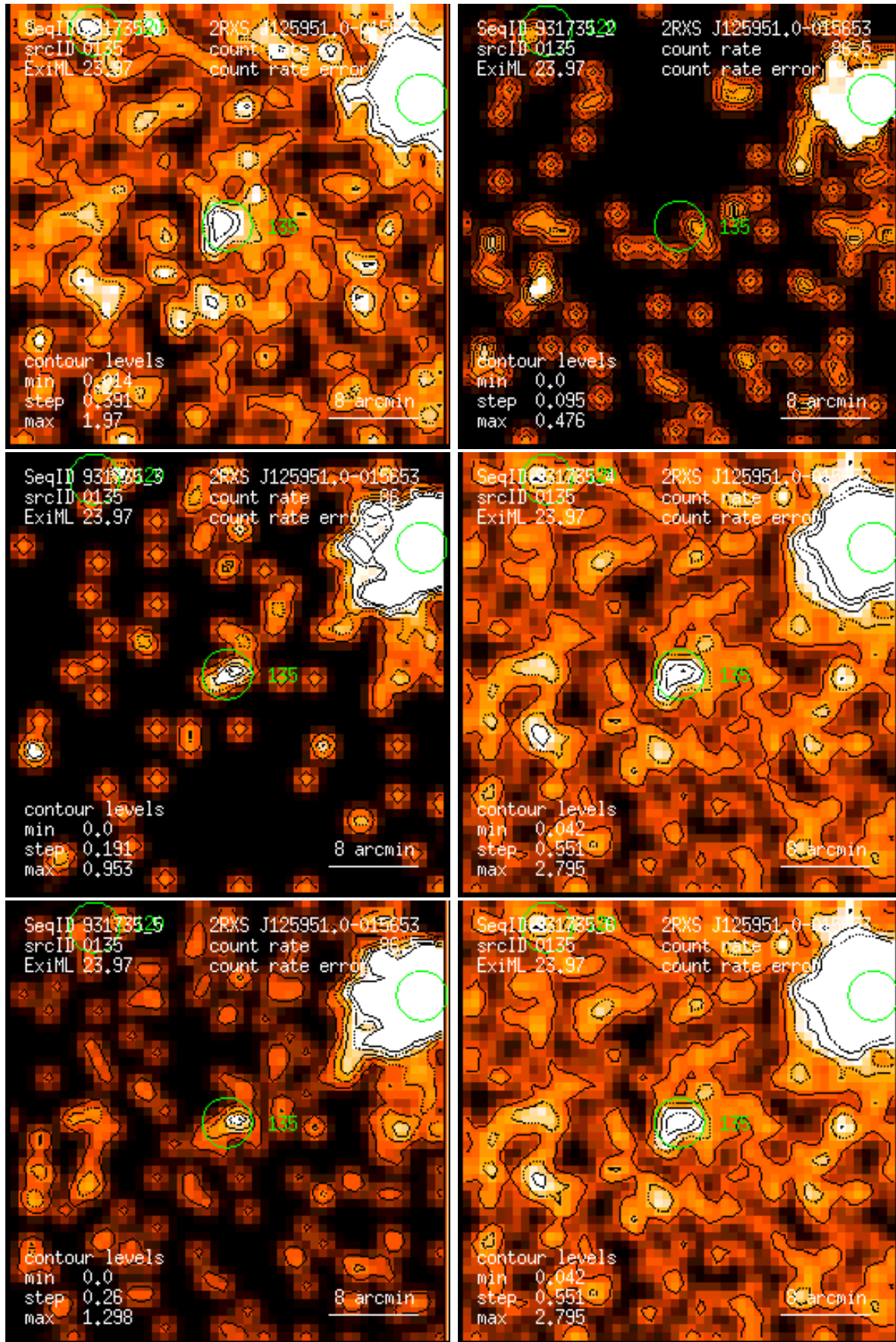
Figure 135: RASS 931735: detection 0135: band rate images, Gaussian filter: (1) PSPC channels 11 – 41, (2) 52 – 90, (3) 91 – 201, (4) 11 – 235, (5) 52 – 201, (6) 11 – 201. Broad band rates in counts/ks. Band rate contour levels in counts/ks/arcmin 2 .
