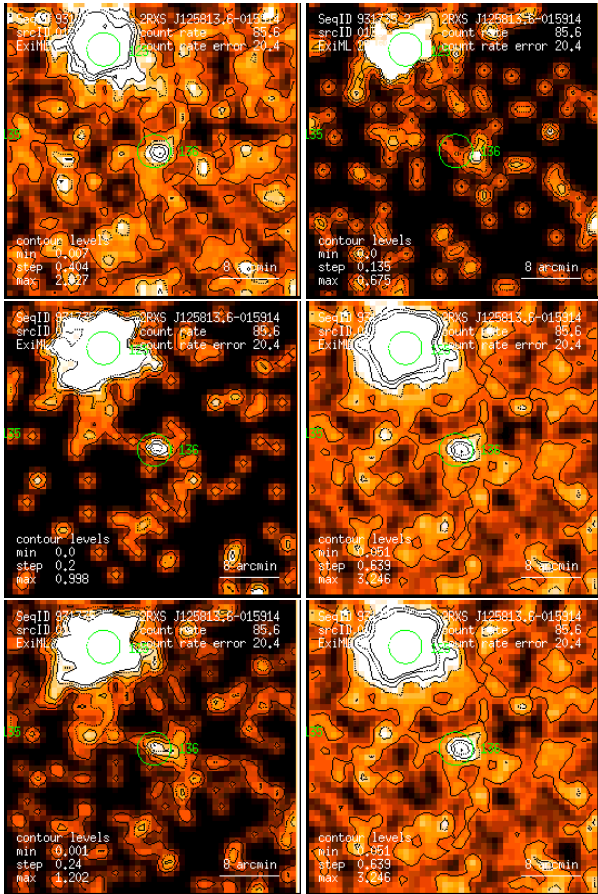
Figure 136: RASS 931735: detection 0136: band rate images, Gaussian filter: (1) PSPC channels 11 – 41, (2) 52 – 90, (3) 91 – 201, (4) 11 – 235, (5) 52 – 201, (6) 11 – 201. Broad band rates in counts/ks. Band rate contour levels in counts/ks/arcmin 2 .
