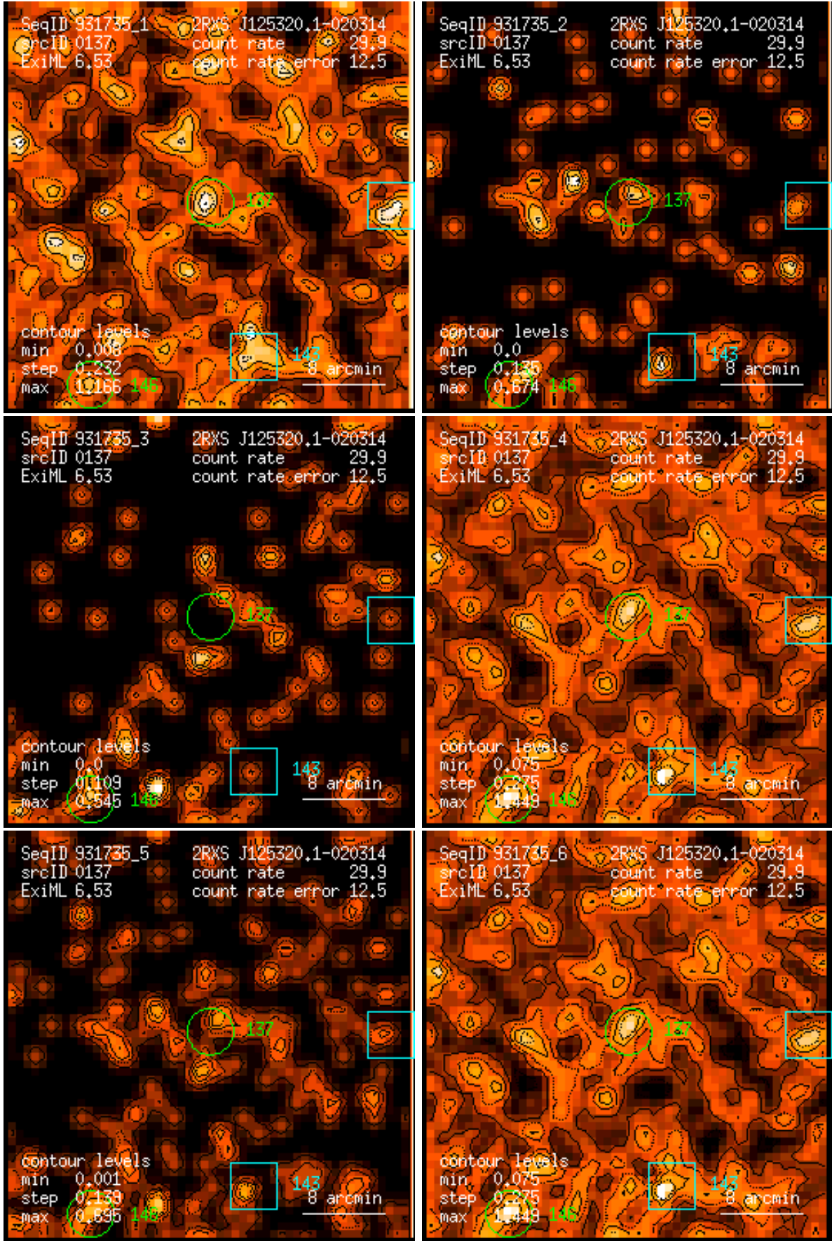
Figure 137: RASS 931735: detection 0137: band rate images, Gaussian filter: (1) PSPC channels 11 – 41, (2) 52 – 90, (3) 91 – 201, (4) 11 – 235, (5) 52 – 201, (6) 11 – 201. Broad band rates in counts/ks. Band rate contour levels in counts/ks/arcmin 2 .
